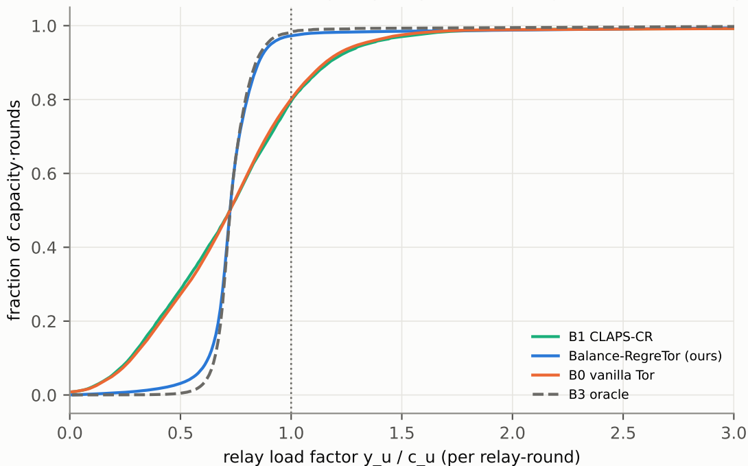
Load factors under random capacity drops (CLAPS weights refreshed hourly)
