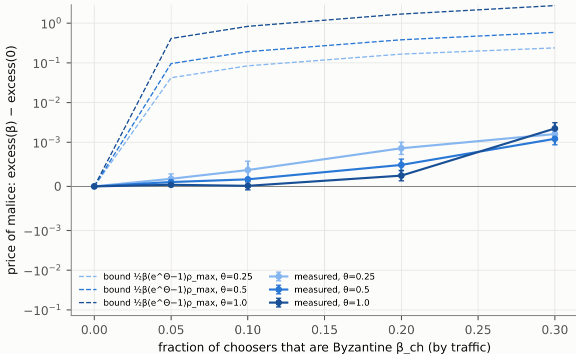
Byzantine choosers skewing lists to colluders (10% of bandwidth)
