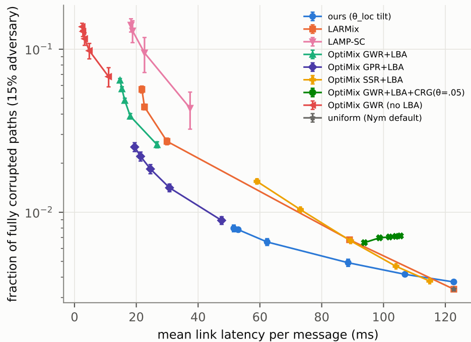
RIPE, \bar{\rho}=0.7 , capacities: equal
