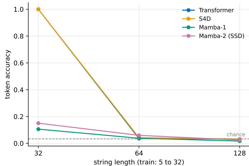
Exact copy: token accuracy vs string length
