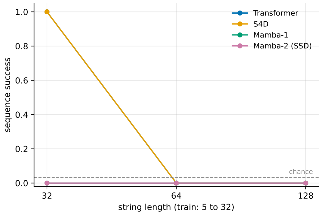
Exact copy: full-sequence success vs length
