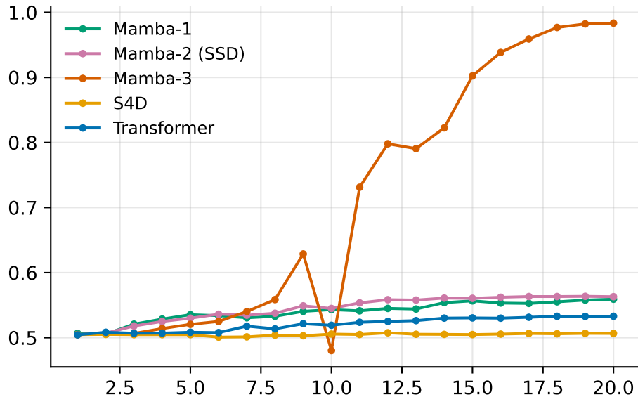
Parity: token accuracy
