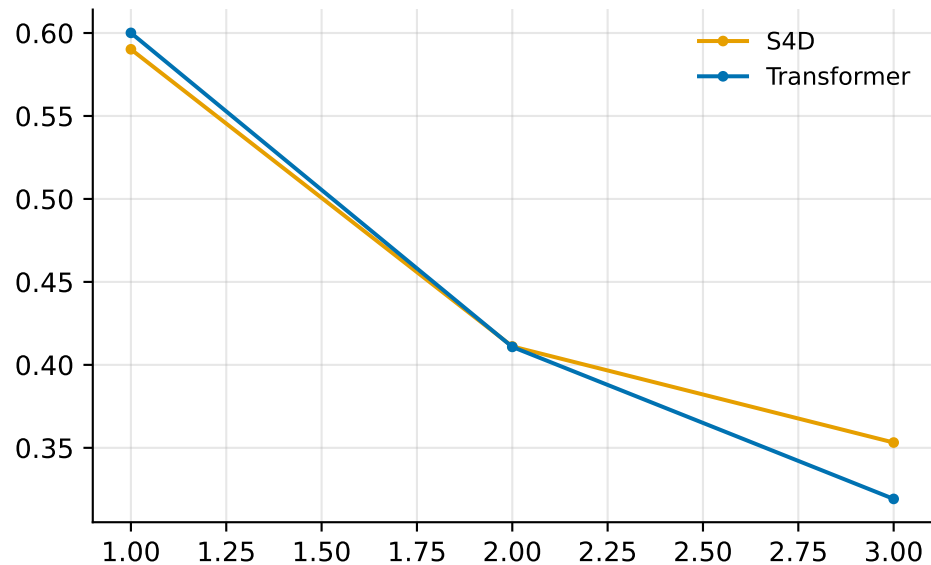
IMDb train loss
