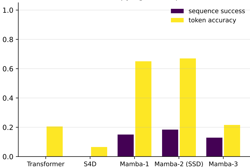
Selective copying (final epoch)
