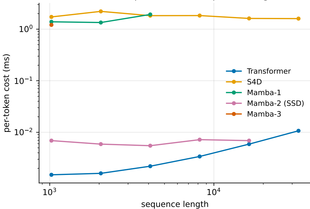
Decode cost per token vs sequence length
