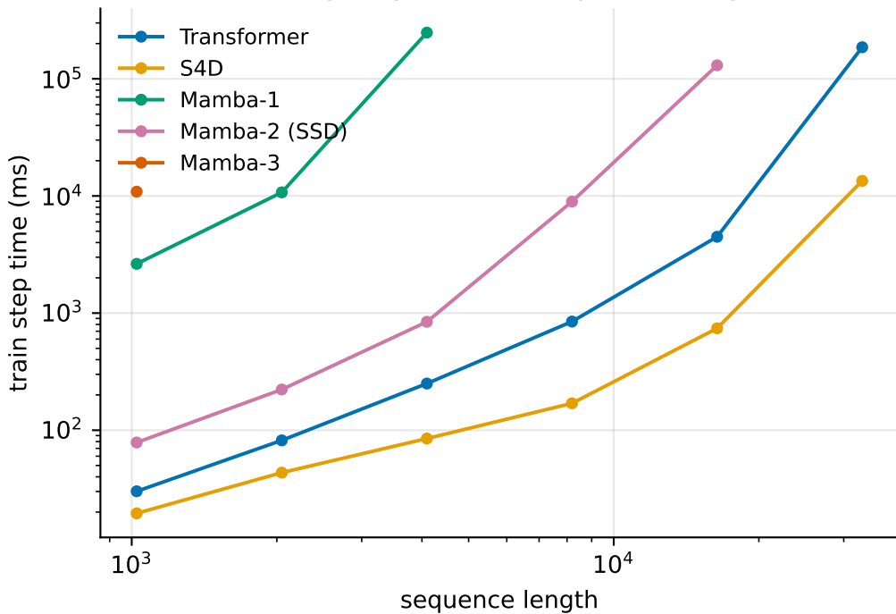
Training step time vs sequence length
