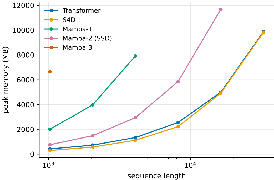
Peak GPU memory vs sequence length
