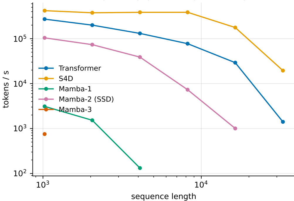
Training throughput vs sequence length
