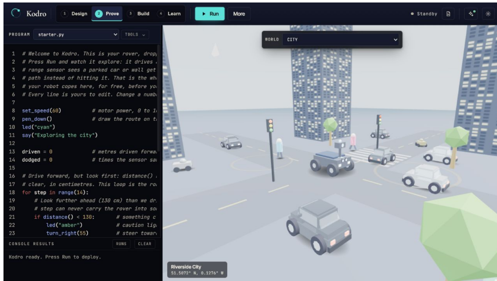
Figure 4.2. The default Simple proving surface. The four-stage journey, one dominant Run action, editable program and three-dimensional city remain visible; secondary actions and the evidence rail are available on demand.
