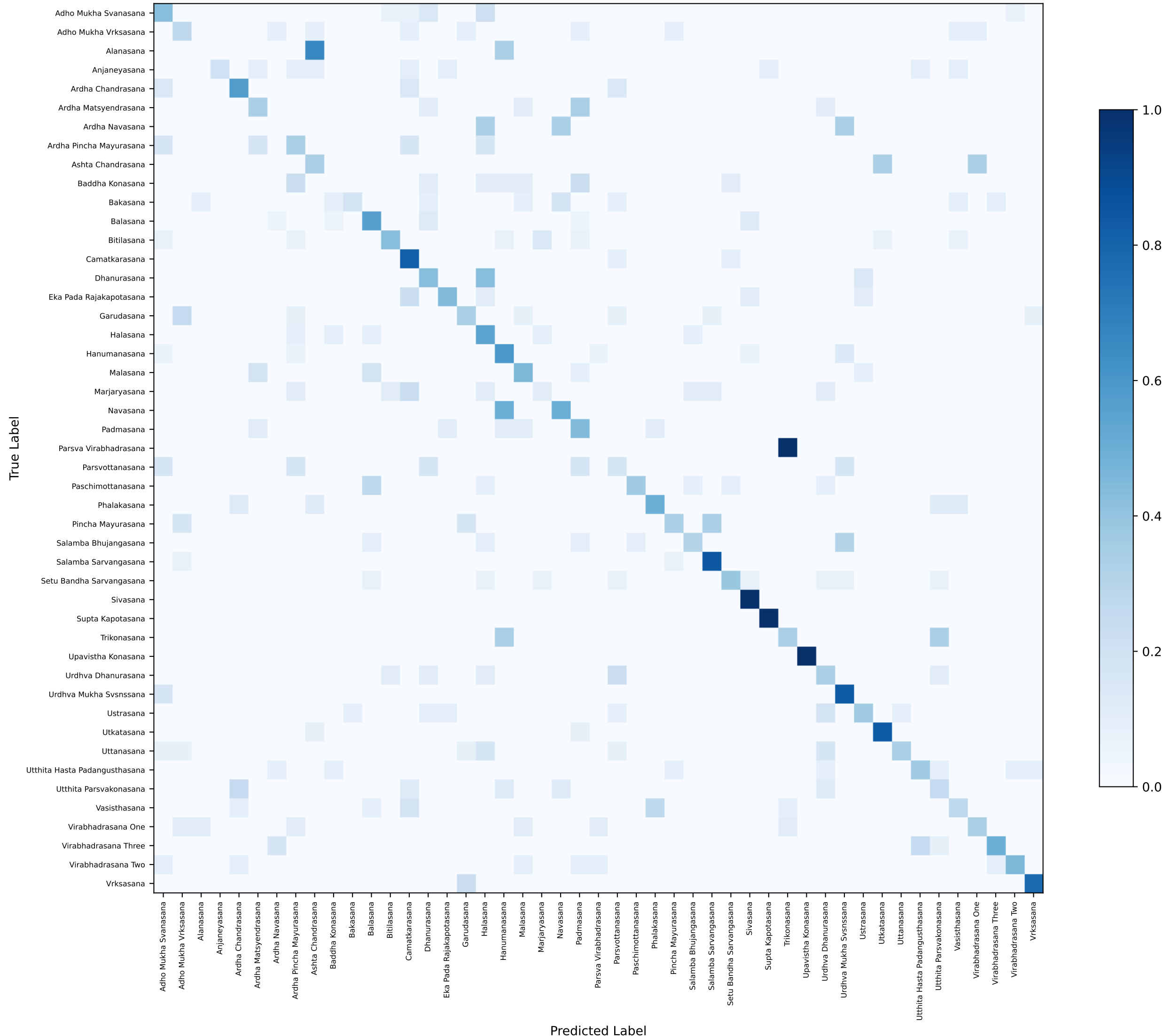
Confusion Matrix (row-normalised) — Custom CNN
