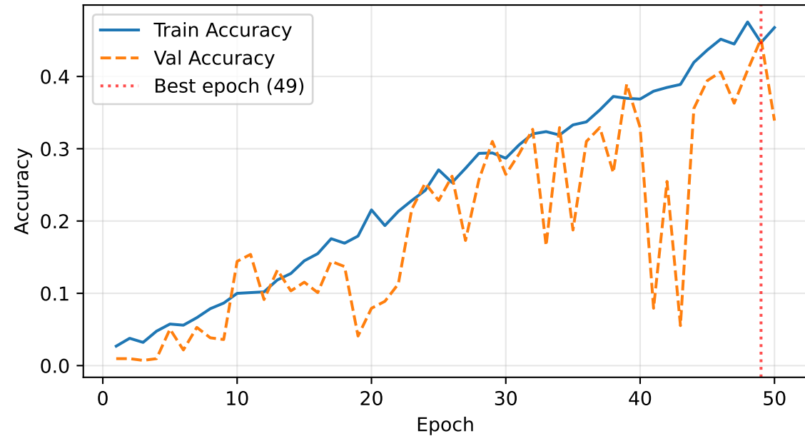
Custom CNN: Accuracy
