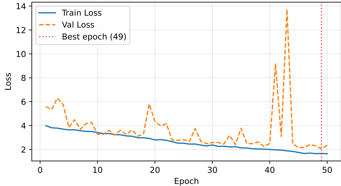
Custom CNN: Loss
