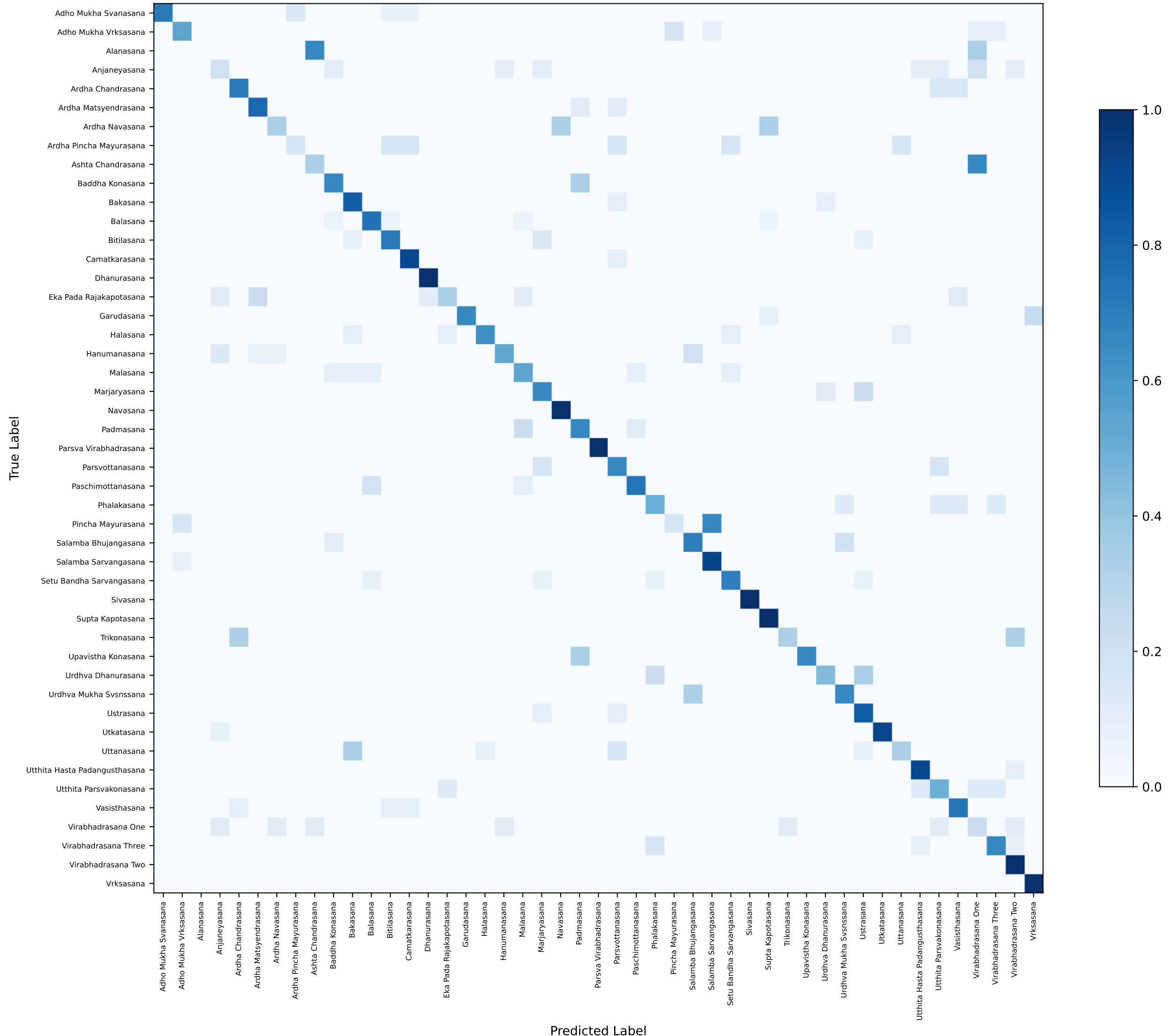
Confusion Matrix (row-normalised) — MobileNetV2
