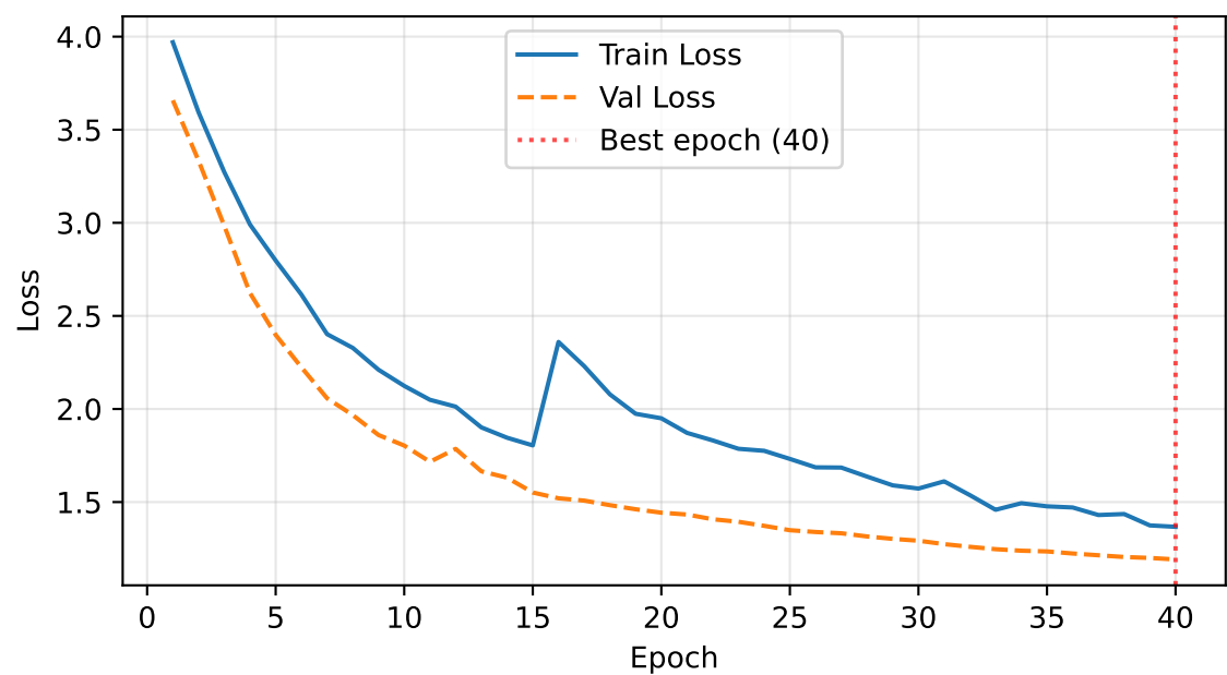
MobileNetV2: Loss
