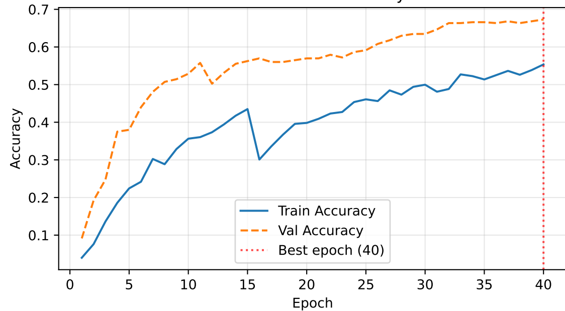
MobileNetV2: Accuracy
