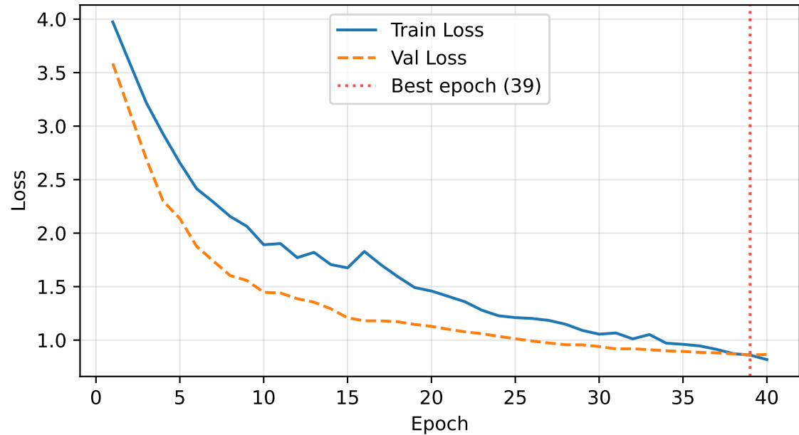
ResNet50: Loss
