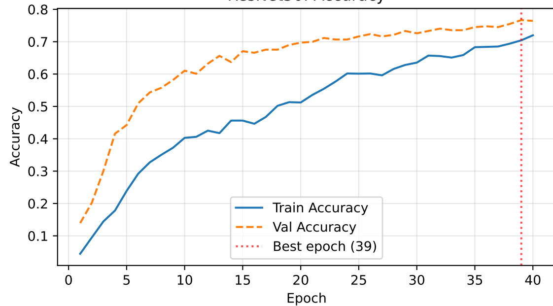
ResNet50: Accuracy
