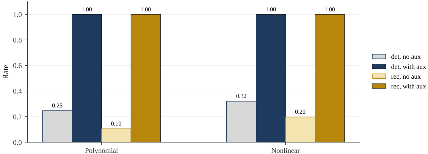
Aux-row ablation: monomial-consistency rows on every slot
