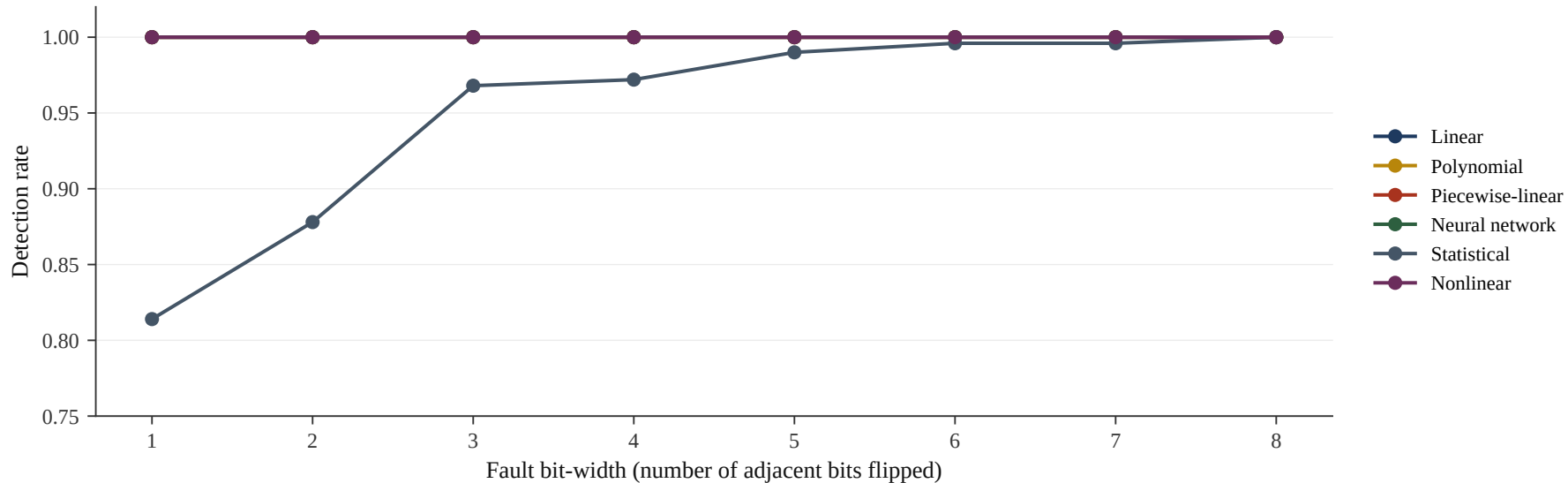
Detection vs spatial cluster size; all frontends at 1.000 except statistical
