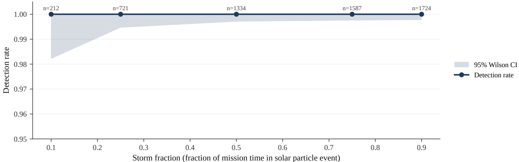
Detection holds under bursty fault regimes (linear frontend, 10 streams x 4h per point)
