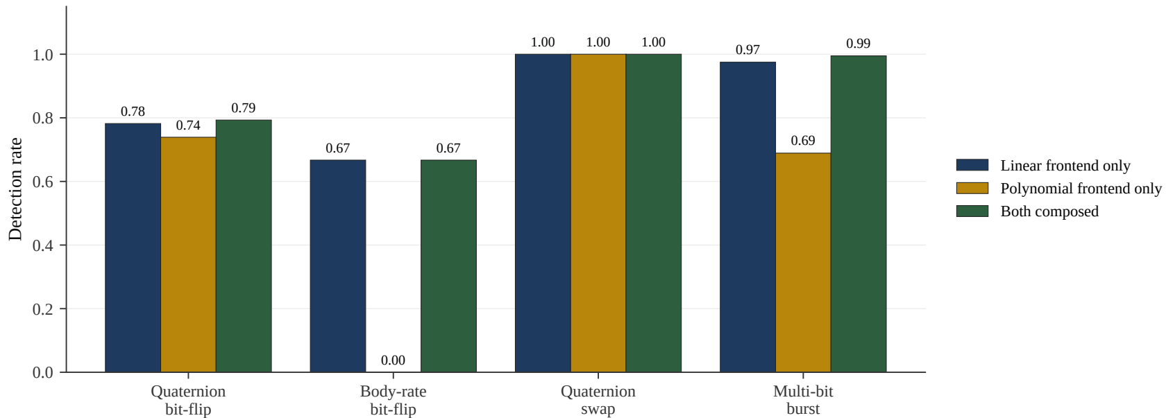
One task, three protection regimes: quaternion attitude controller
