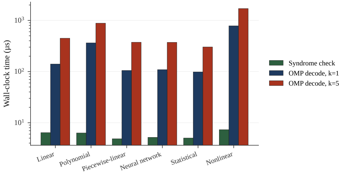
Per-call latency on x86-64 Linux
