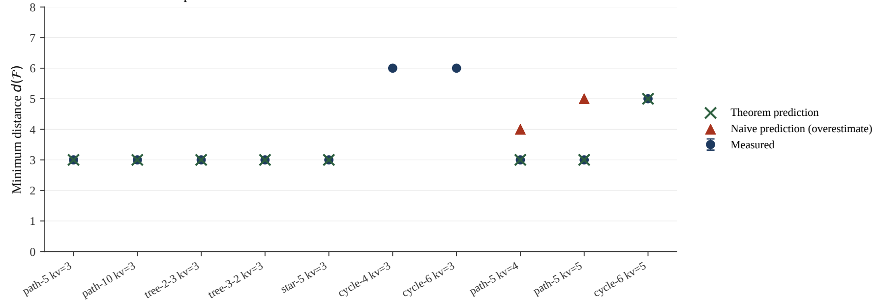
Altitude bound: theorem prediction vs measured distance
