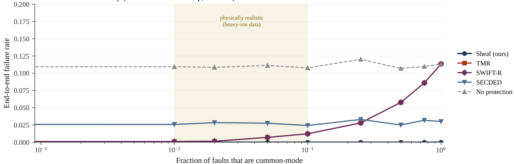
Common-mode sensitivity (total fault rate 0.001/op, N=5000)
