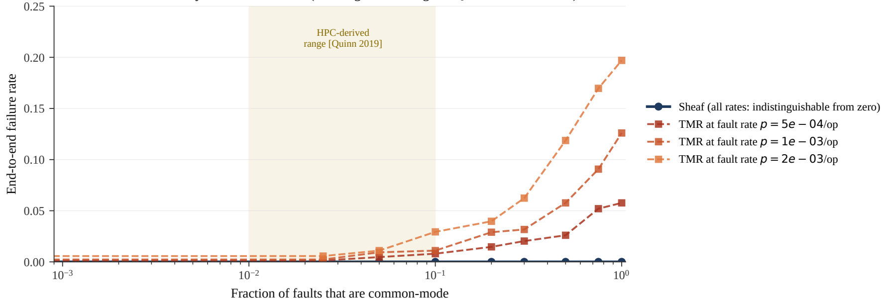
Common-mode sensitivity at three fault rates (4× range bracketing the Quinn et al.\ estimate)
