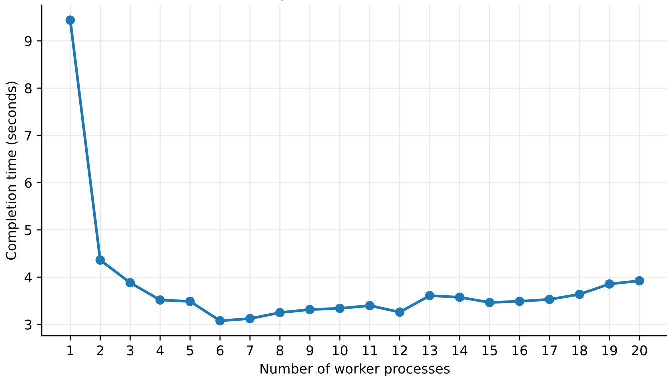
Crawl Completion Time vs Worker Count
