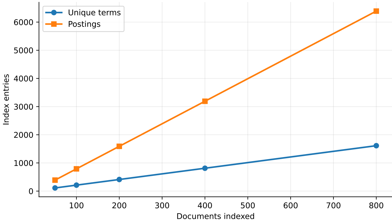
Inverted Index Growth vs Document Count
