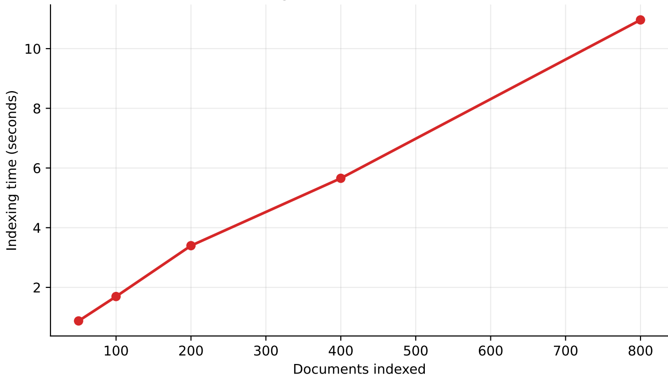
Indexing Time vs Document Count
