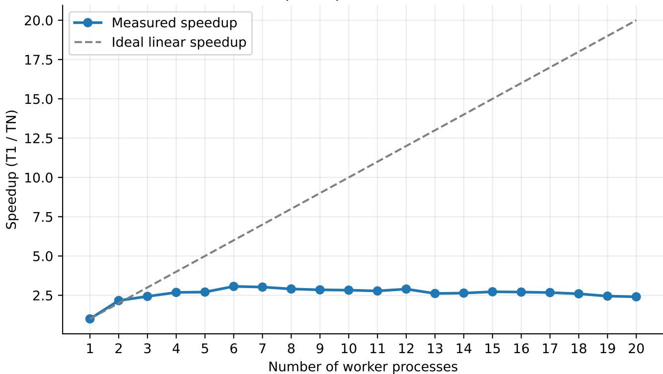
Measured Speedup Relative to One Worker
