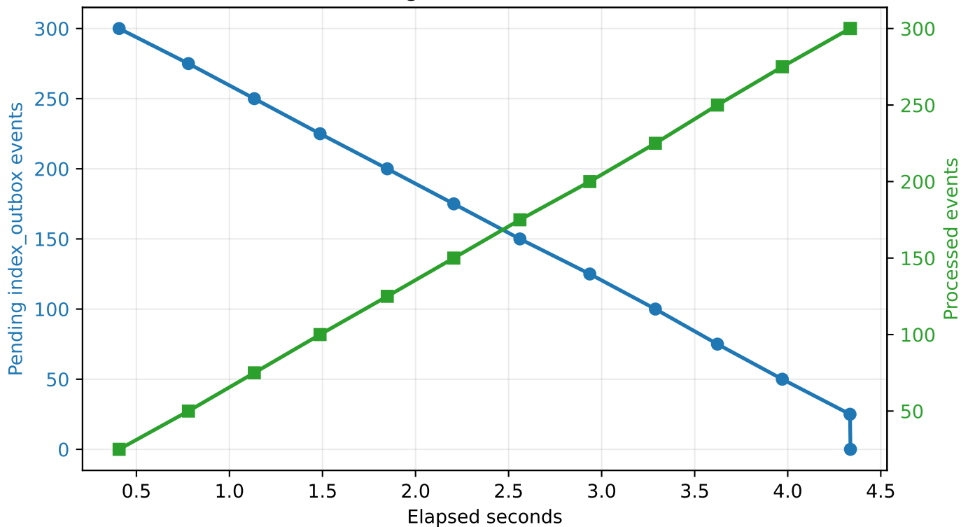
Streaming Indexer Outbox Drain
