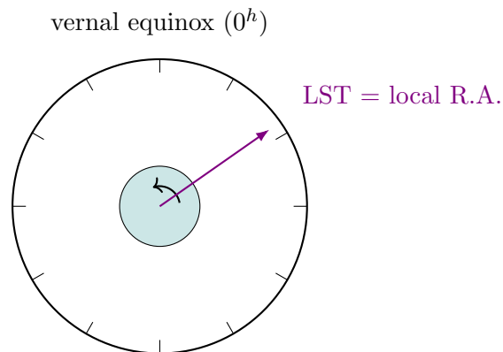
Figure 5: The R.A. “clock face” stays fixed against the stars while the Earth (center) turns underneath it. The arrow marks whichever R.A. value currently coincides with the observer's local meridian — that value is the LST.
