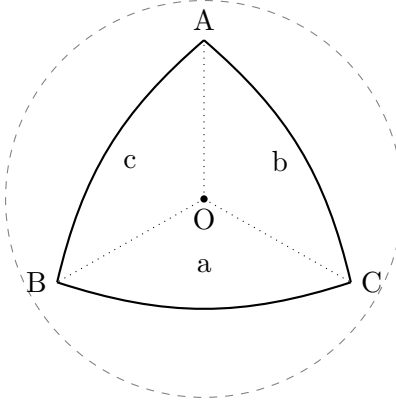
Figure 9: A spherical triangle. The dashed circle is the sphere itself; the solid curved arcs a , b , c are arcs of great circles on that sphere's surface, and O is the sphere's center. Lower-case letters name the arc lengths (equivalently, the central angles: the arc a = \angle BOC ), and upper-case letters name the vertex angles — \angle A is the angle between the planes AOB and AOC .
