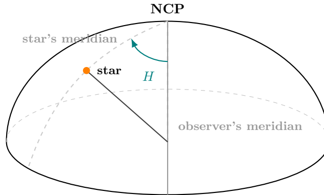
Figure 4: Hour angle H . The zero-value of H is when the star sits exactly on the observer's local meridian; H then grows as the star drifts west, which is the natural direction to treat as “forward in time,” since stars rise in the east and set in the west.
