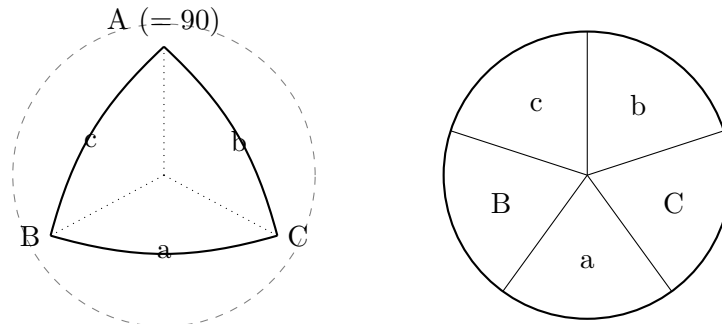
Figure 12: Left — a right spherical triangle, with the curved sides drawn exactly as in Figure 9, just with one vertex ( A ) fixed at 90. Right — Napier's circle: the five other angular elements of the triangle (everything except the known 90 angle), arranged around a wheel in the same order they appear going around the triangle.
