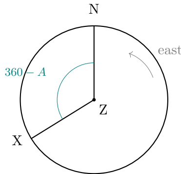
Figure 11: A flat top-down view of the observer's horizon, used only to pin down the azimuth convention. Since azimuth increases eastward while our triangle's vertex angle at Z opens the other way, \angle Z = 360 - A .
