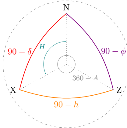
Figure 10: The spherical triangle NXZ that connects the north celestial pole, a celestial object, and the observer's zenith. This one triangle is the entire bridge between horizontal and equatorial coordinates.
