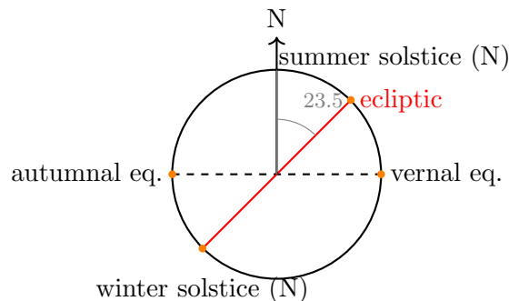
Figure 3: The Sun’s declination over the year, shown as the tilt of the ecliptic (the Sun’s apparent path) against the celestial equator. At the summer solstice the Sun sits at its northernmost declination ( +23.5^\circ , over the tropic of cancer); at the winter solstice its southernmost ( -23.5^\circ , over the tropic of capricorn); the convention flips for the southern hemisphere. At either equinox the Sun crosses the celestial equator, \delta = 0 .
