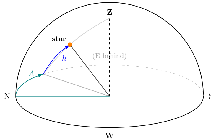
Figure 1: The observer's sky bubble. The altitude h is measured from the horizon up to the zenith Z (0–90); the azimuth A is measured along the horizon from north, going east (0–360).
