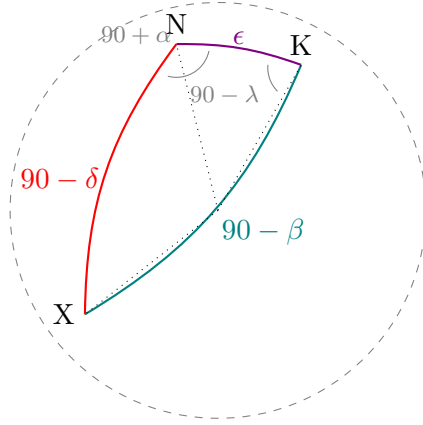
Figure 13: The spherical triangle connecting the celestial pole N , the ecliptic pole K , and an object X . The tilt angle \epsilon sits right between the two poles.
