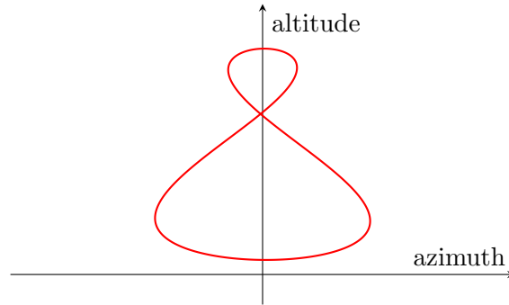
Figure 14: The analemma — the figure-eight traced on the sky by the Sun’s position at the same clock time every day of the year, a direct visual record of the equation of time (its east-west width) combined with the seasonal swing in declination (its north-south length).
