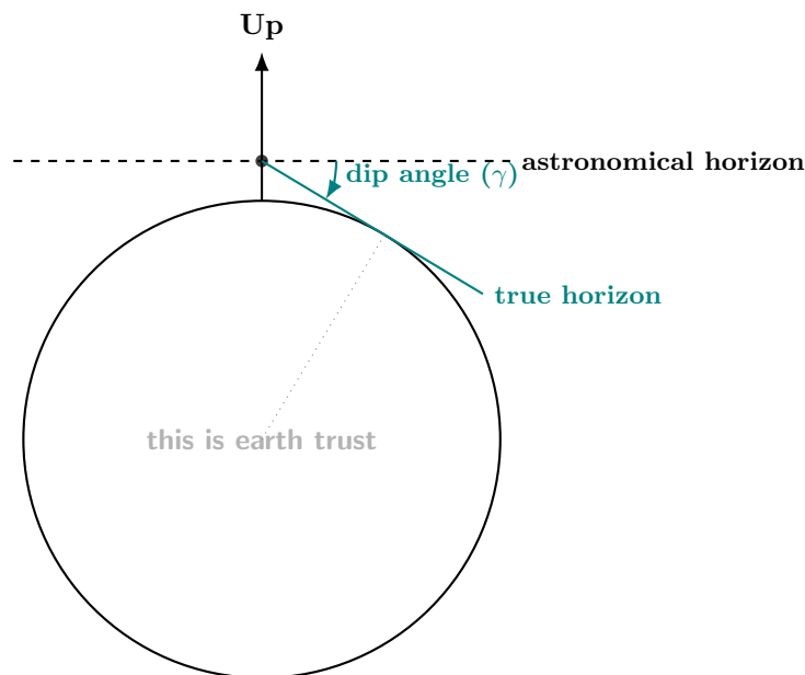
Figure 8: The dip angle. From height h above sea level (the gray dot, raised above the Earth's surface), the observer's true horizon — the line of sight that just grazes the Earth's curve — dips below the eye-level astronomical horizon.
