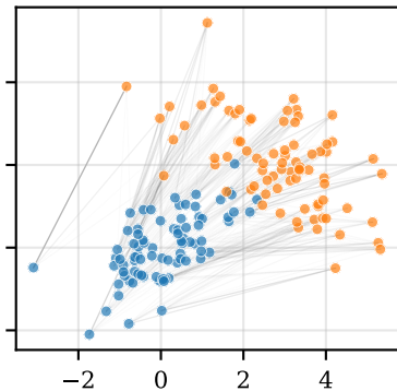
Sinkhorn, \lambda = 1
