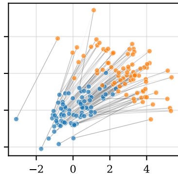
Sinkhorn, \lambda = 0.05
