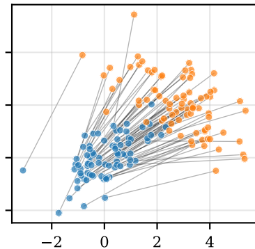
Quadratic, \lambda = 0.05
