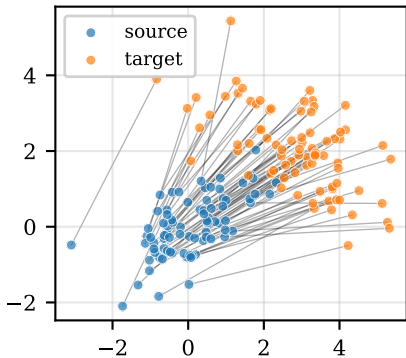
LP (exact)
