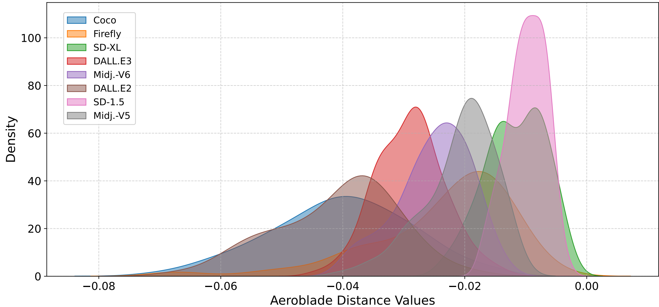
KDE of Aeroblade Distance Values
