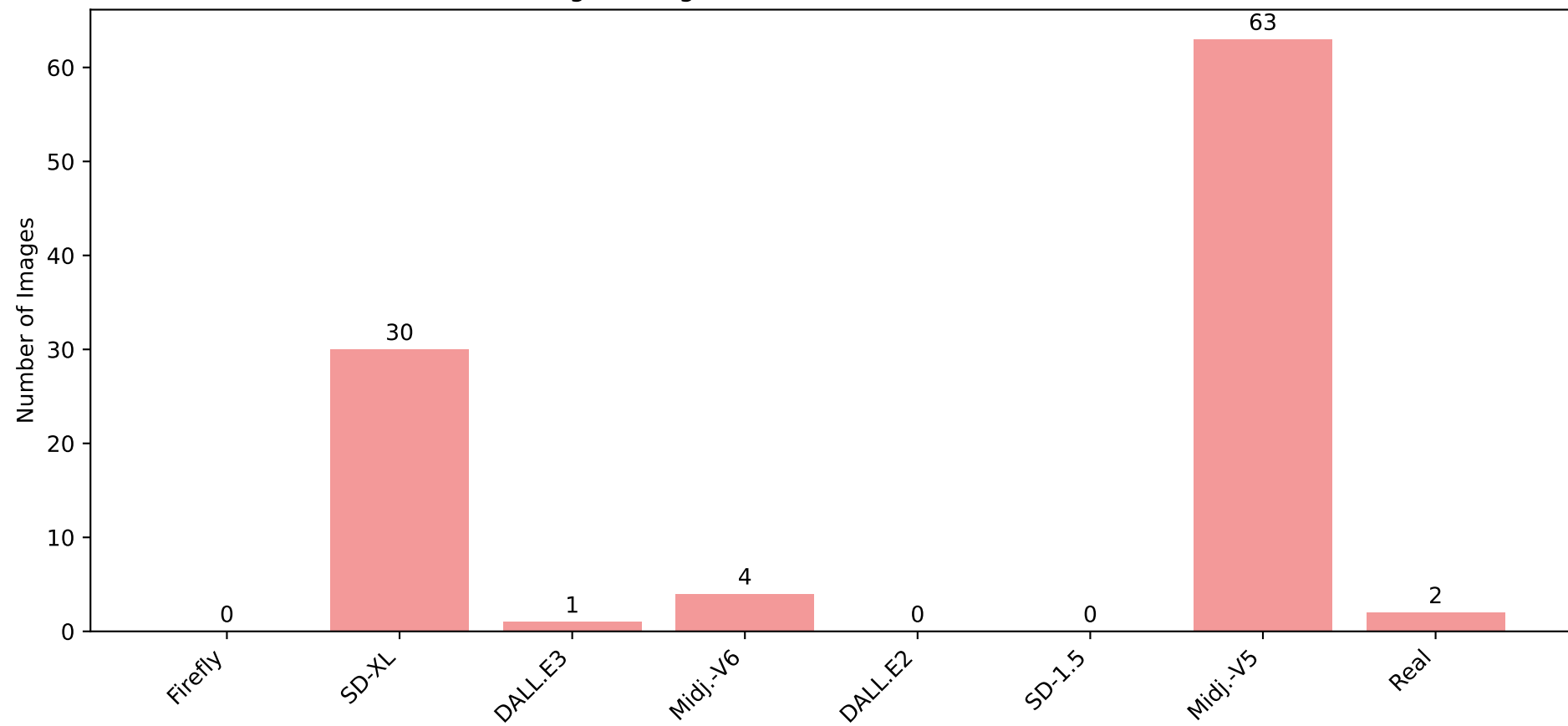
Flux Images Assigned to Known Generators (SREC Prior)
