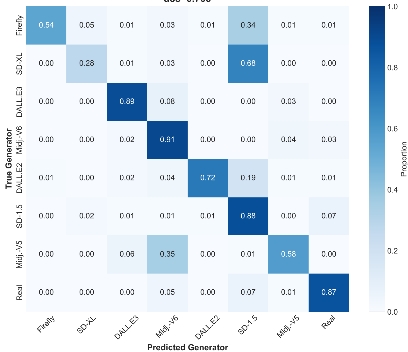
Confusion Matrix (Row-Normalized) acc=0.709
