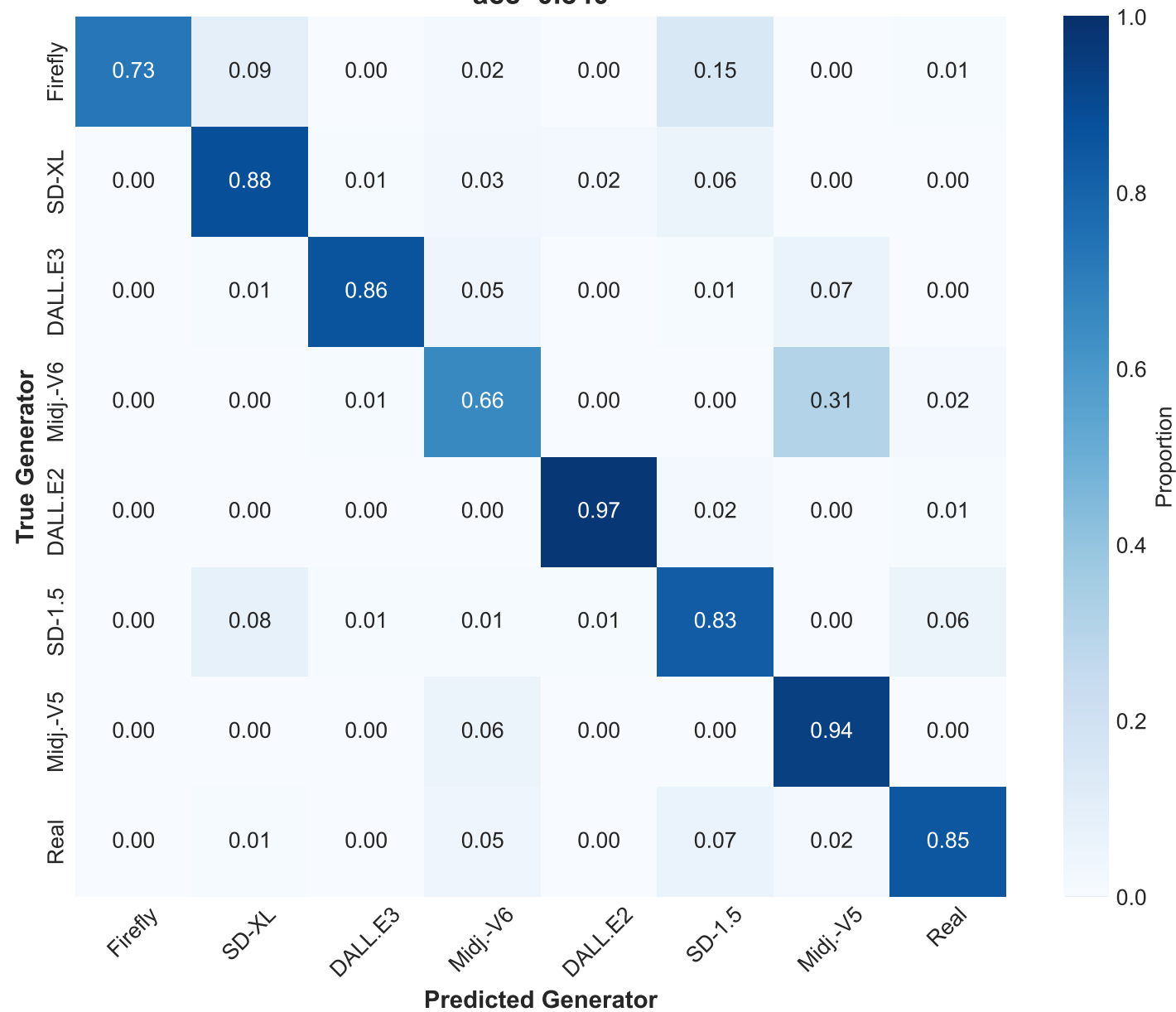
Confusion Matrix (Row-Normalized) acc=0.840
