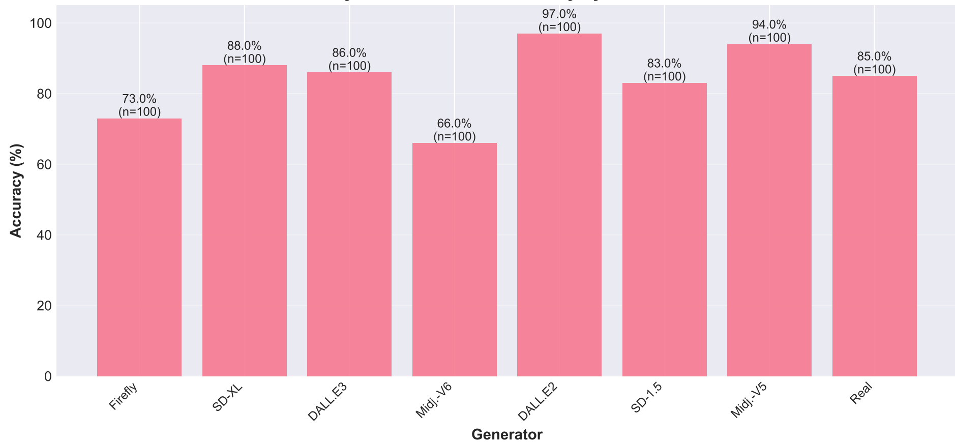
Bayesian Attribution Accuracy by Generator
