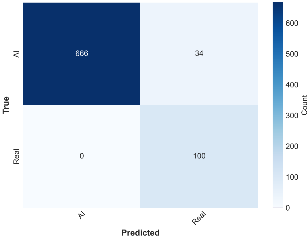
Real vs AI (Counts) acc=0.958
