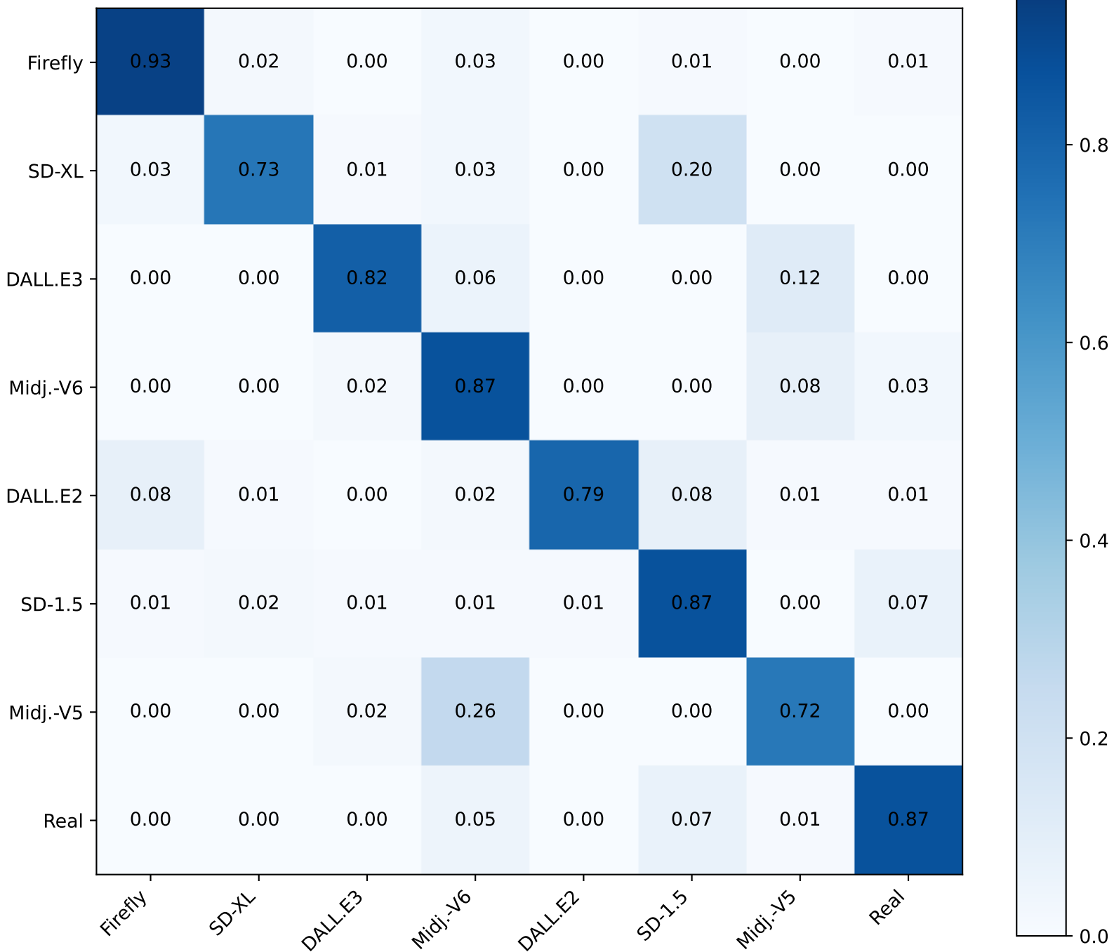
confusion matrix (row-normalized) acc=82.50%
