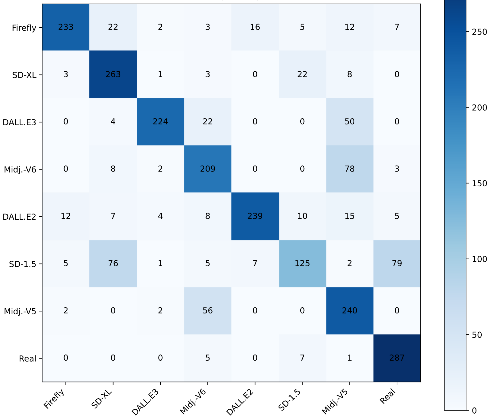
confusion matrix (counts) acc=75.83%
