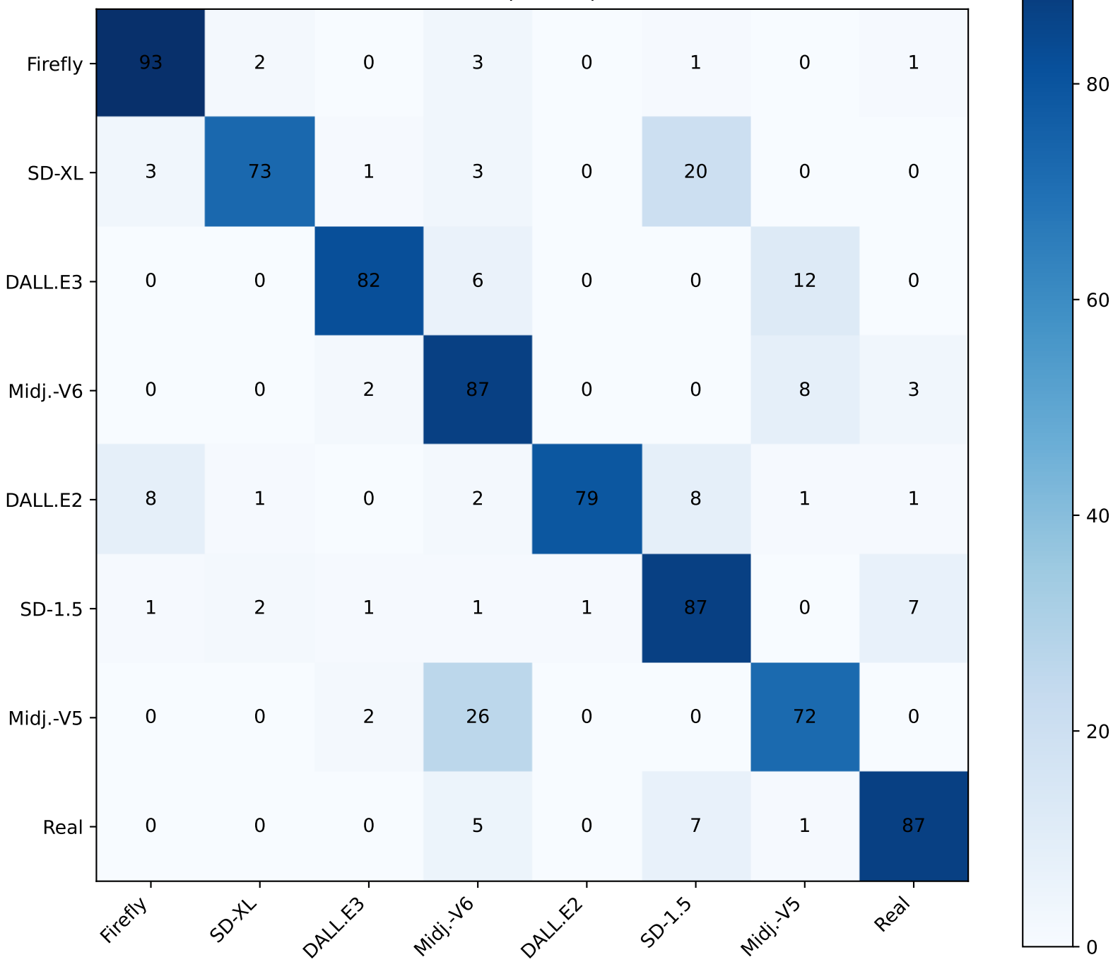
confusion matrix (counts) acc=82.50%
