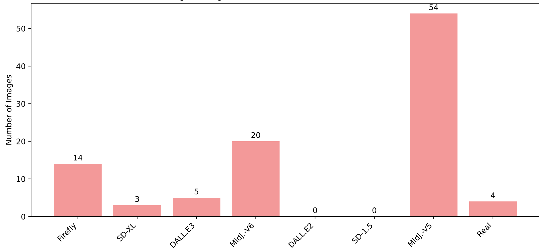
Flux Images Assigned to Known Generators (AEROBLADE Prior)
