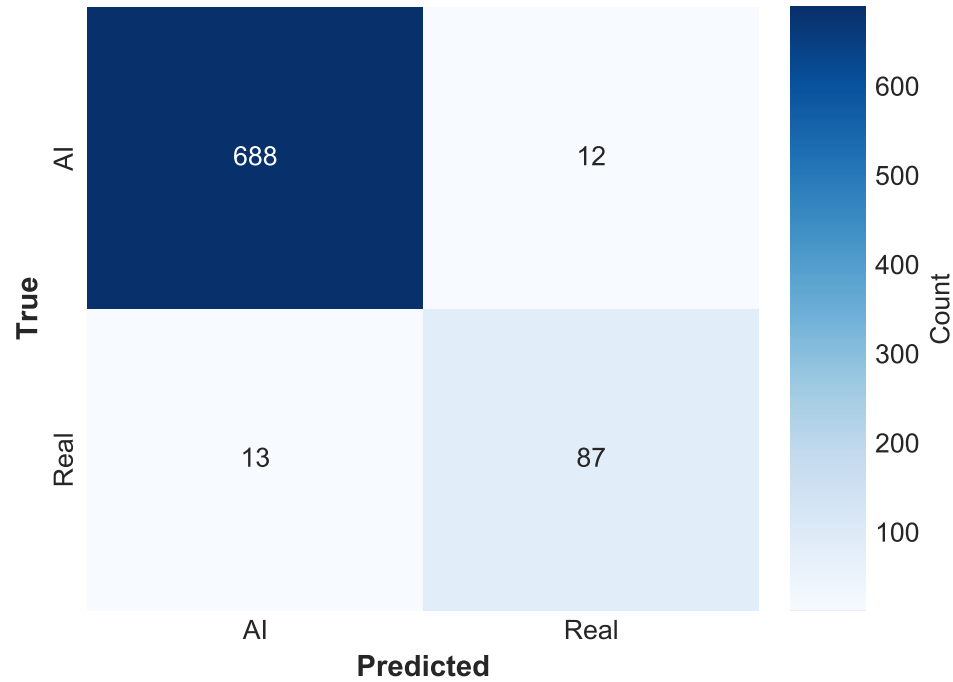
Real vs AI (Counts) acc=0.969
