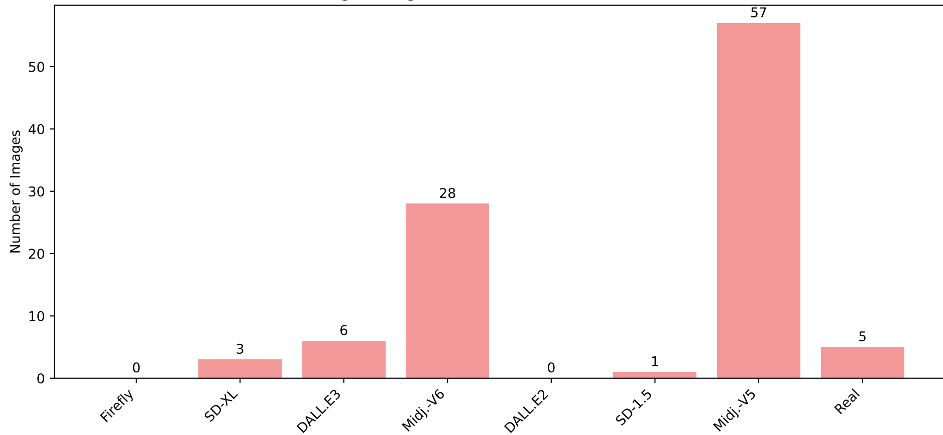
Flux Images Assigned to Known Generators (RIGID Prior)
