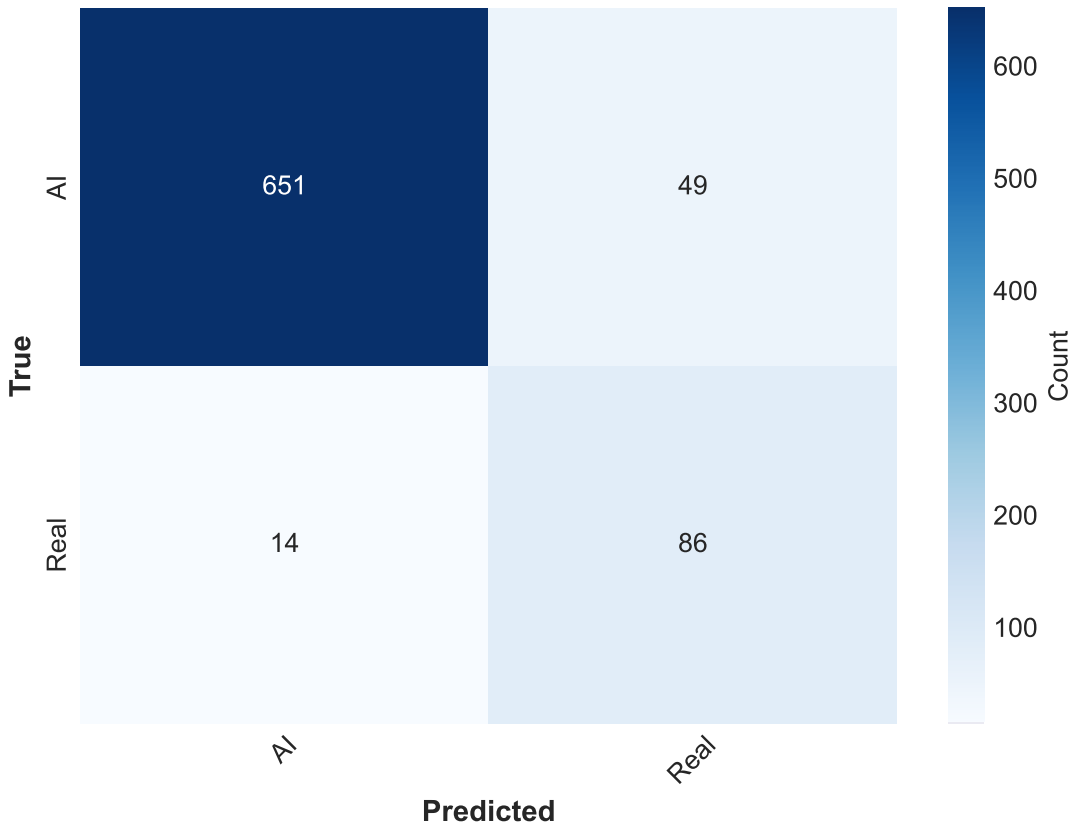
Real vs AI (Counts) acc=0.921
