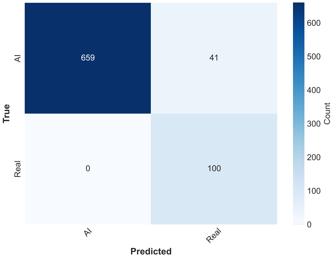
Real vs AI (Counts) acc=0.949
