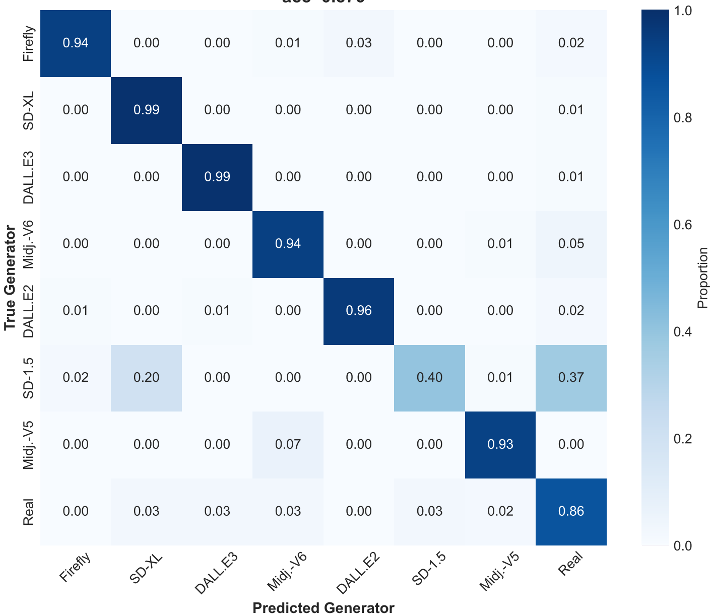
Confusion Matrix (Row-Normalized) acc=0.876
