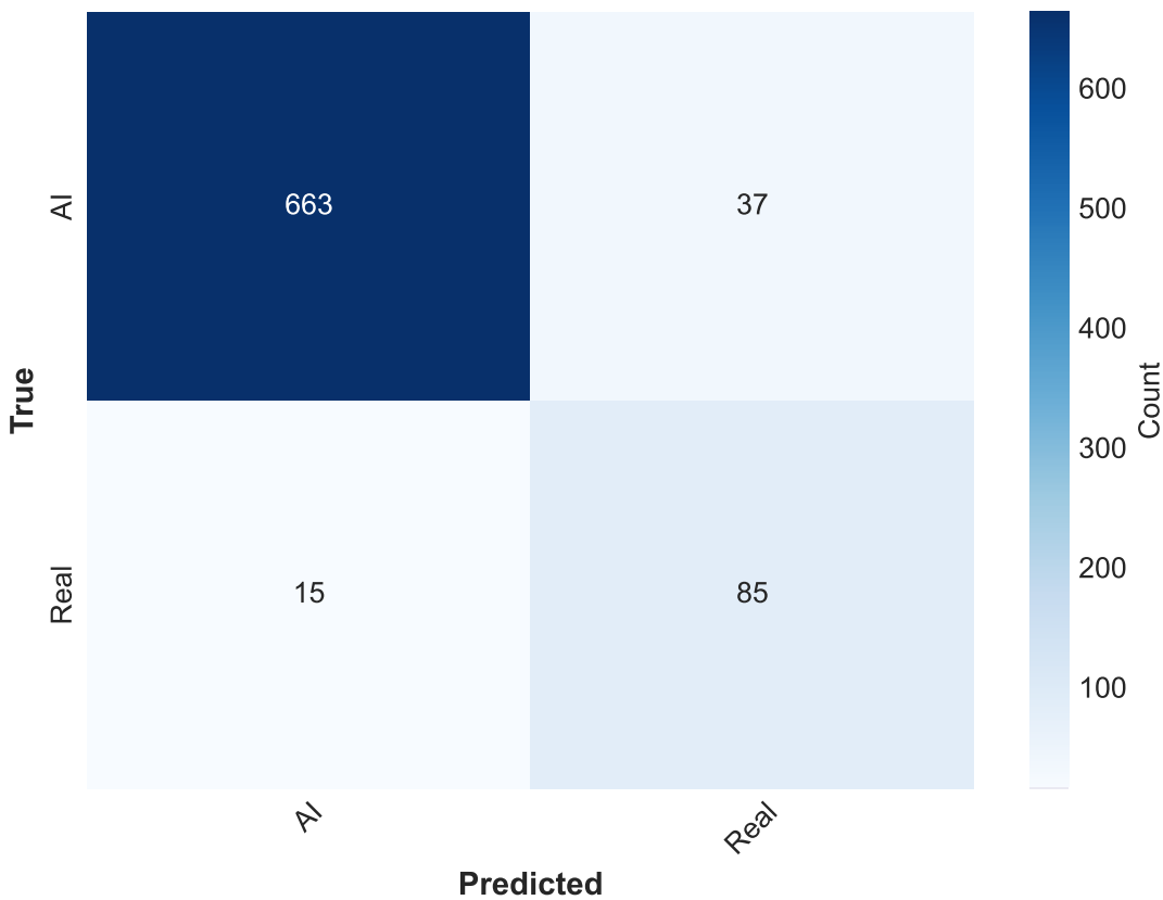
Real vs AI (Counts) acc=0.935
