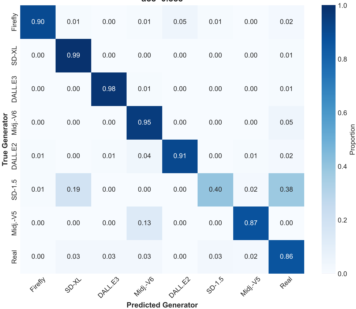
Confusion Matrix (Row-Normalized) acc=0.858
