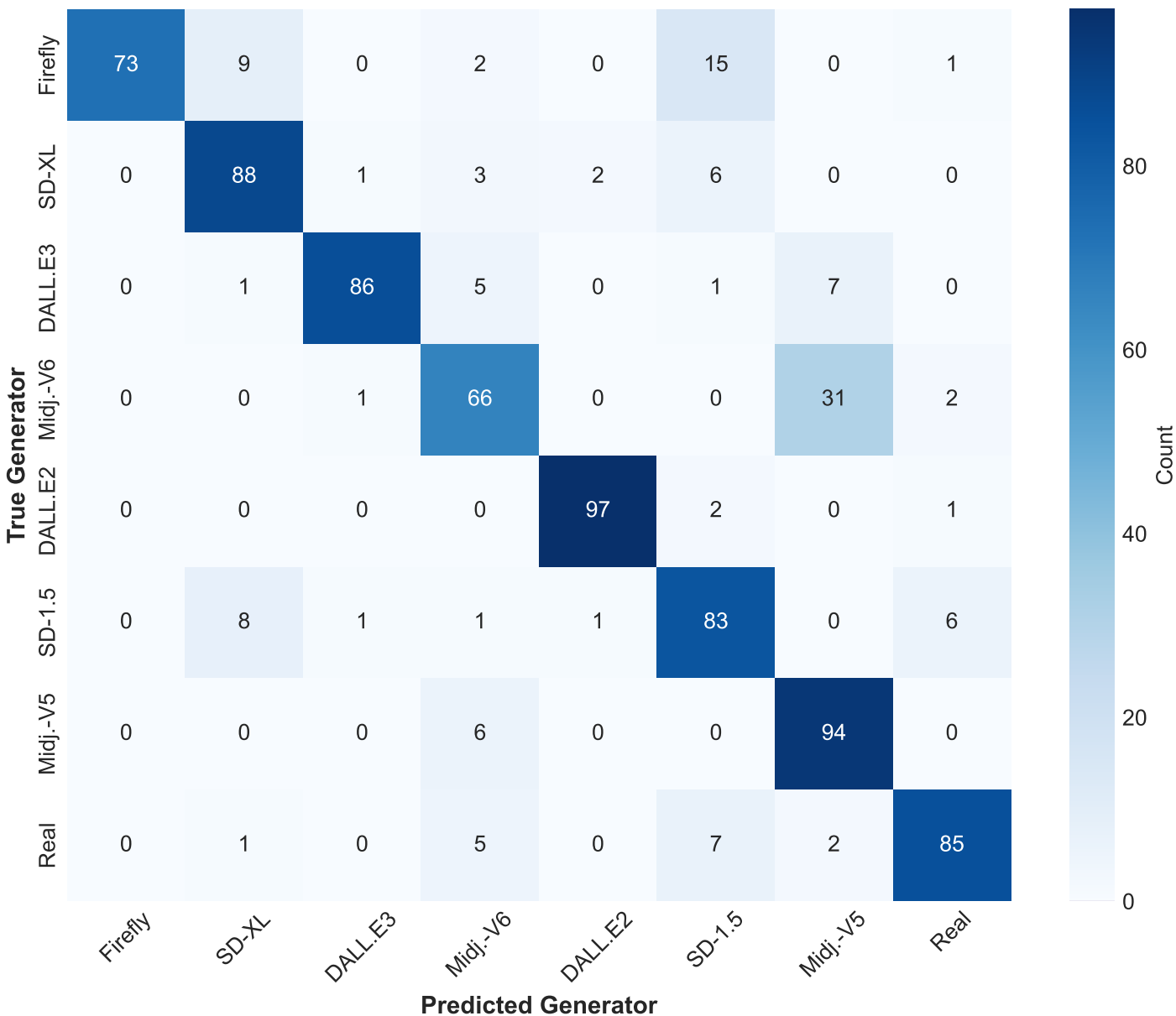
Confusion Matrix (Counts) acc=0.840
