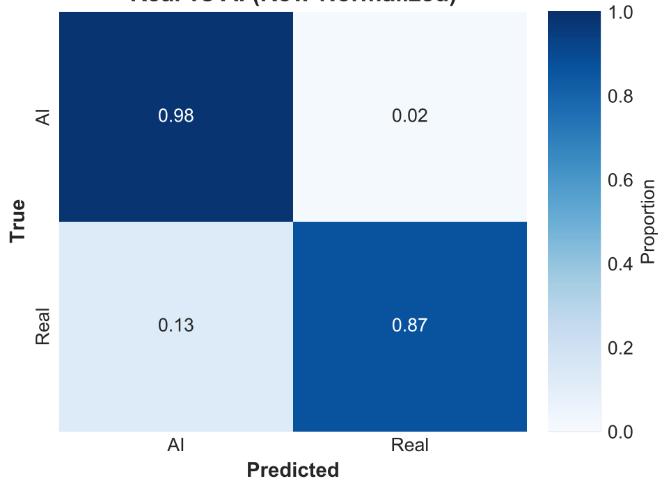
Real vs AI (Row-Normalized)
