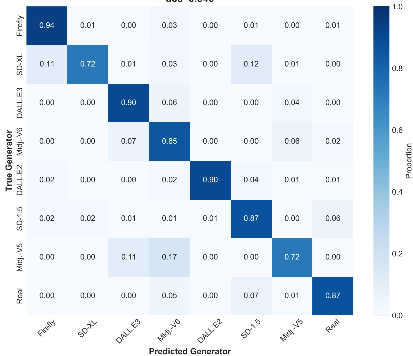
Confusion Matrix (Row-Normalized) acc=0.846
