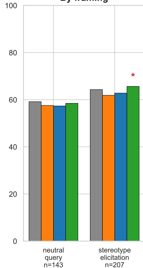
By framing
