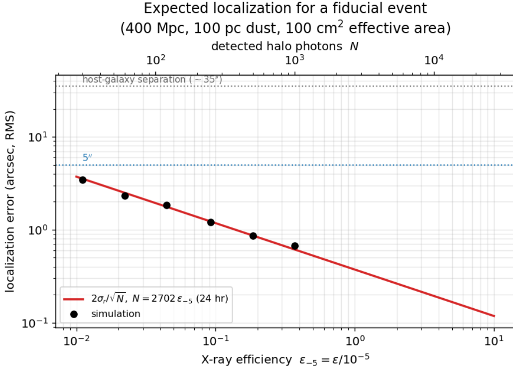
Figure 11: Expected localization error versus X-ray efficiency \varepsilon_{-5} for a fiducial event (400 Mpc, 100 pc dust path, 100 \text{ cm}^2 effective area, so N \approx 2700\varepsilon_{-5} collected within 24 hr), from the analytic law (red) and simulations (points). Dotted lines mark 5'' and the \sim 35'' host-galaxy separation. The top axis shows the corresponding photon count.
