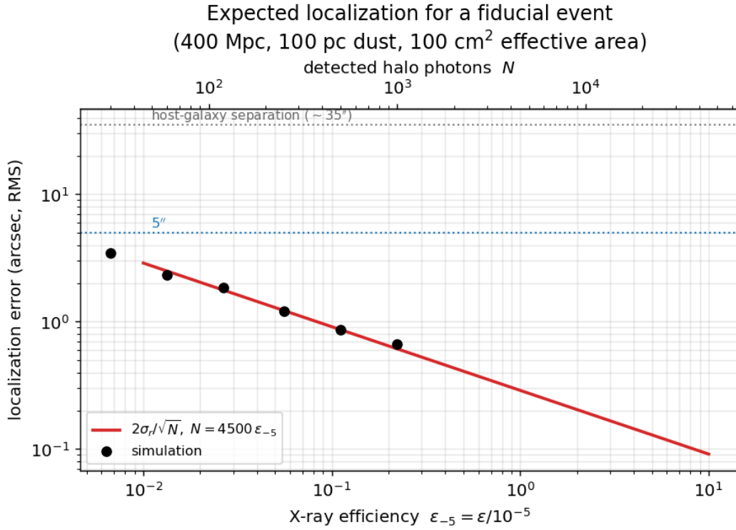
Figure 11: Expected localization error versus X-ray efficiency \epsilon_{-5} for a fiducial event (400 Mpc, 100 pc dust path, 100 cm 2 effective area, so N \approx 4500\epsilon_{-5} over the halo lifetime), from the analytic law (red) and simulations (points). Dotted lines mark 5'' and the \sim 35'' host-galaxy separation. The top axis shows the corresponding photon count.
