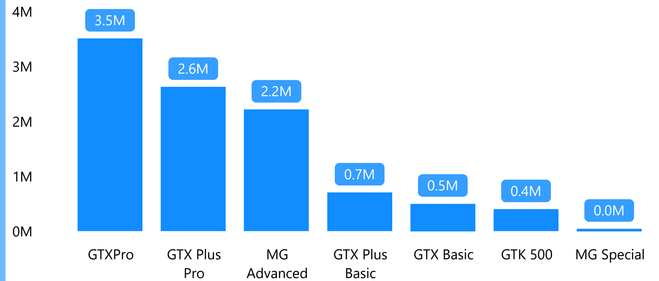
Total_revenue by product
