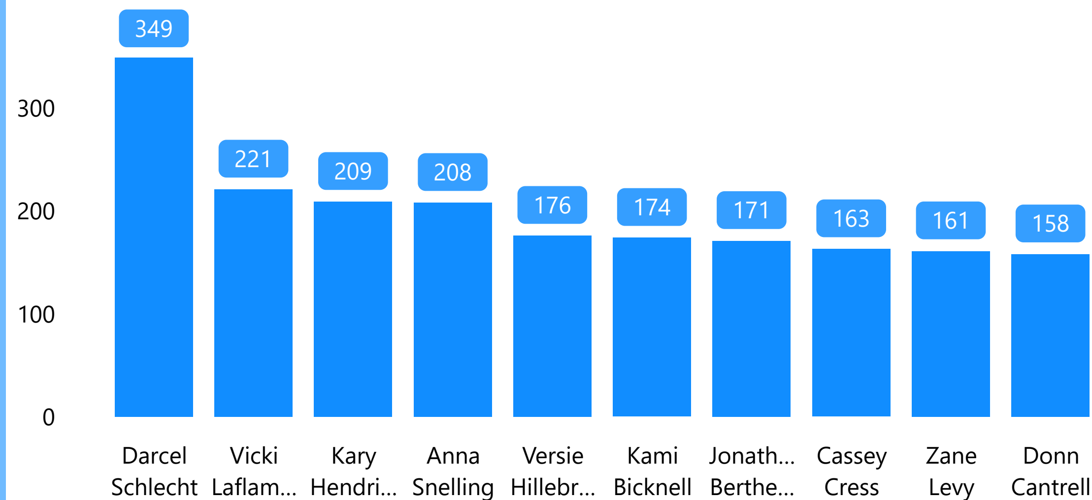
deals_won by sales_agent
