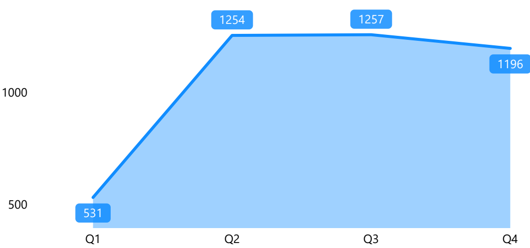
Deal_closed_count by Quarter
