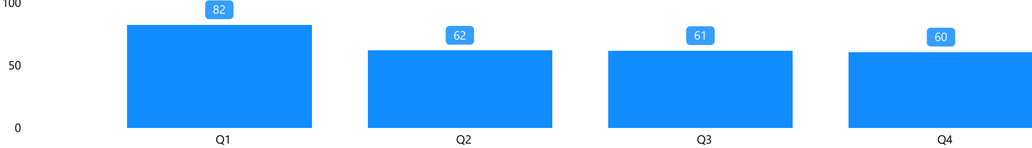
win_rate(%) by Quarter
