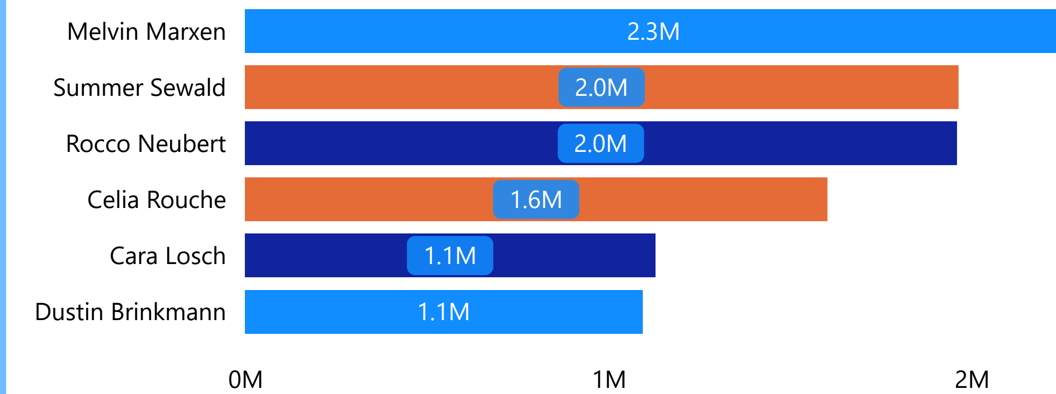
deals_won by sales_agent
