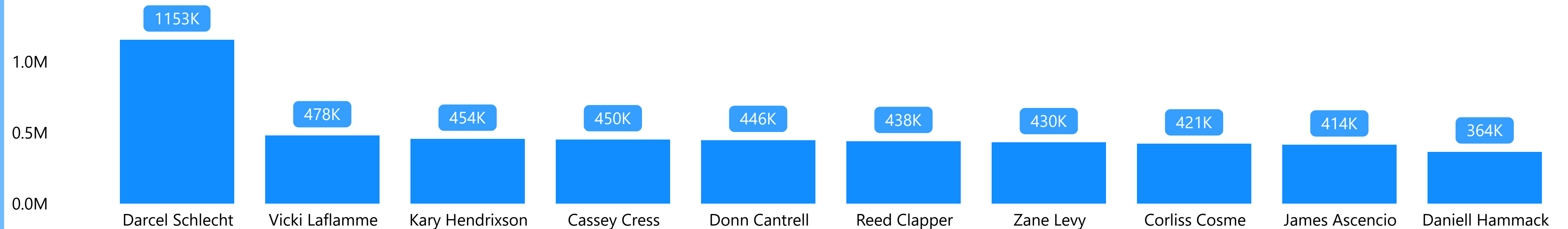
Total_revenue by sales_agent
