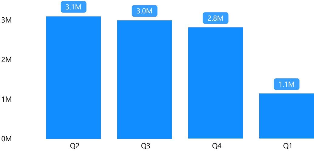
Total_revenue by Quarter
