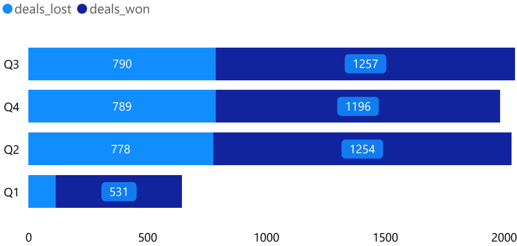
deals_lost and deals_won by Quarter
