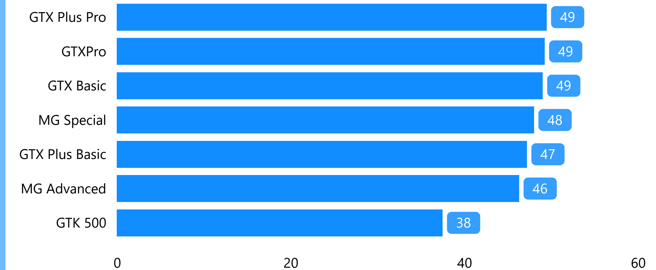
win_rate(%) by product
