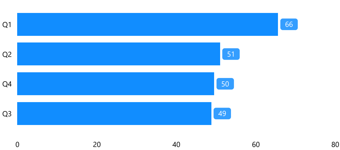
Avg_time_to_close(Days) by Quarter
