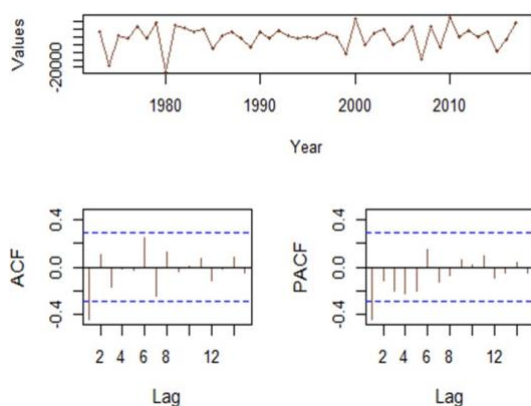
Canada - ACF & PACF after 2 Differencing
