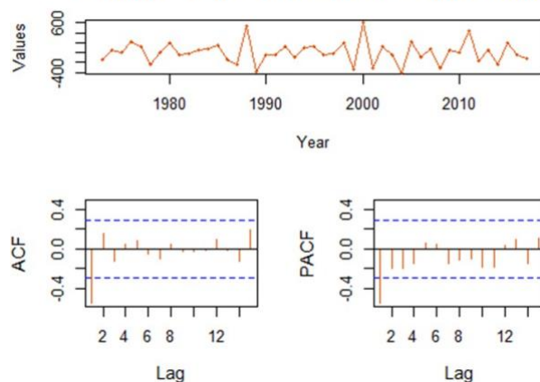
German - ACF & PACF after 2 Differencing
