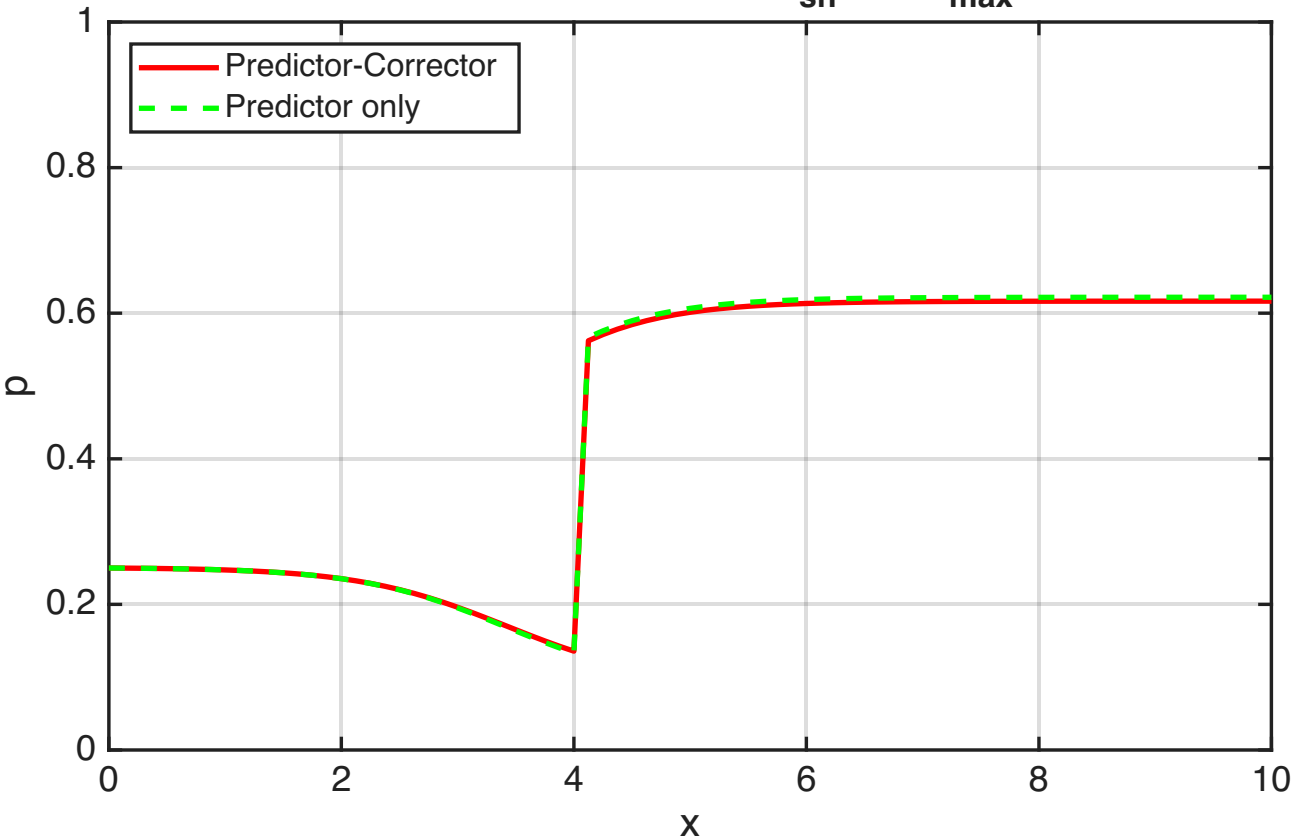
Space Marching: p vs. x ( x_{sh}=4.0, j_{max}=81 )
