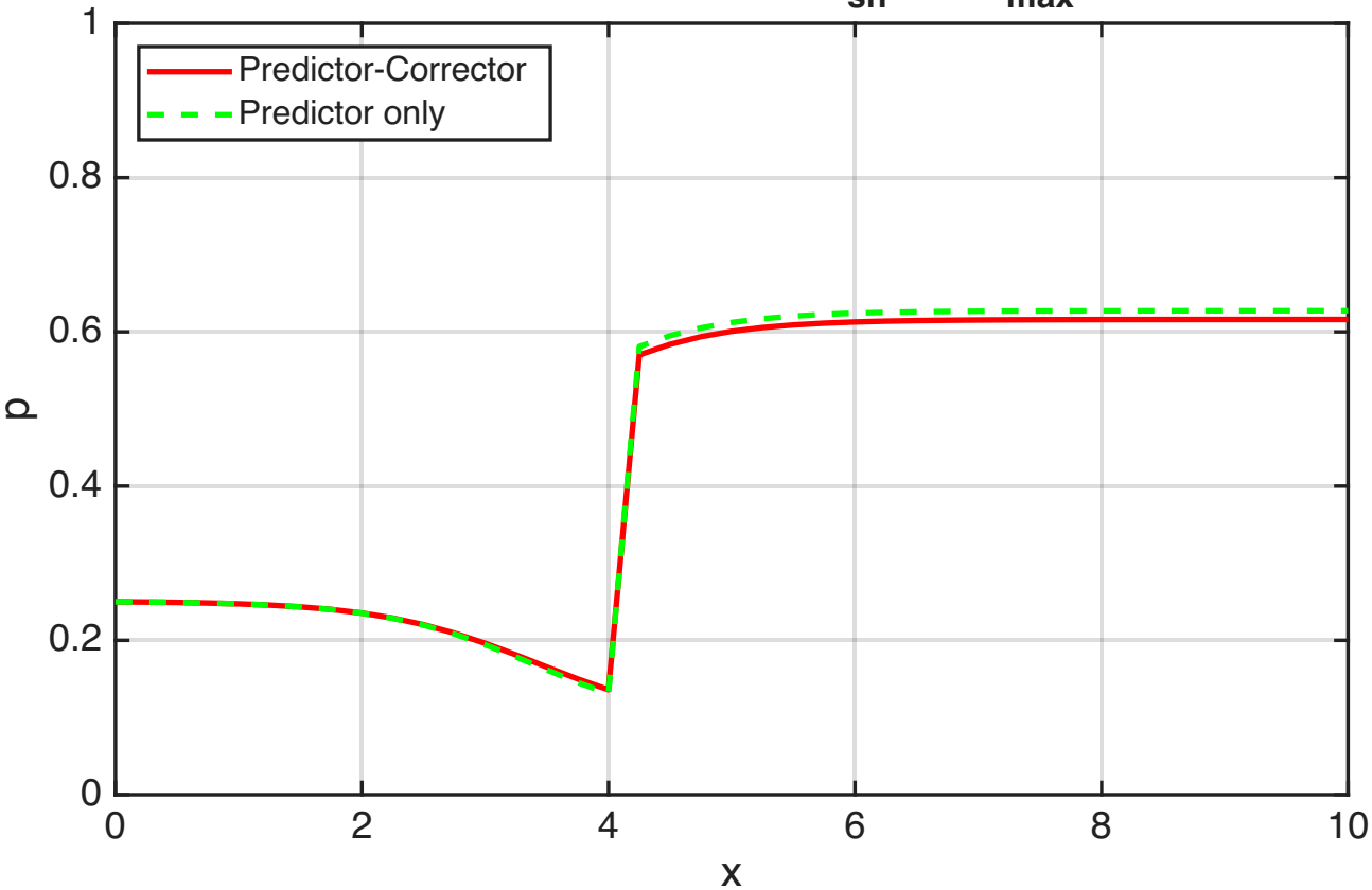
Space Marching: p vs. x ( x_{sh}=4.0, j_{max}=41 )
