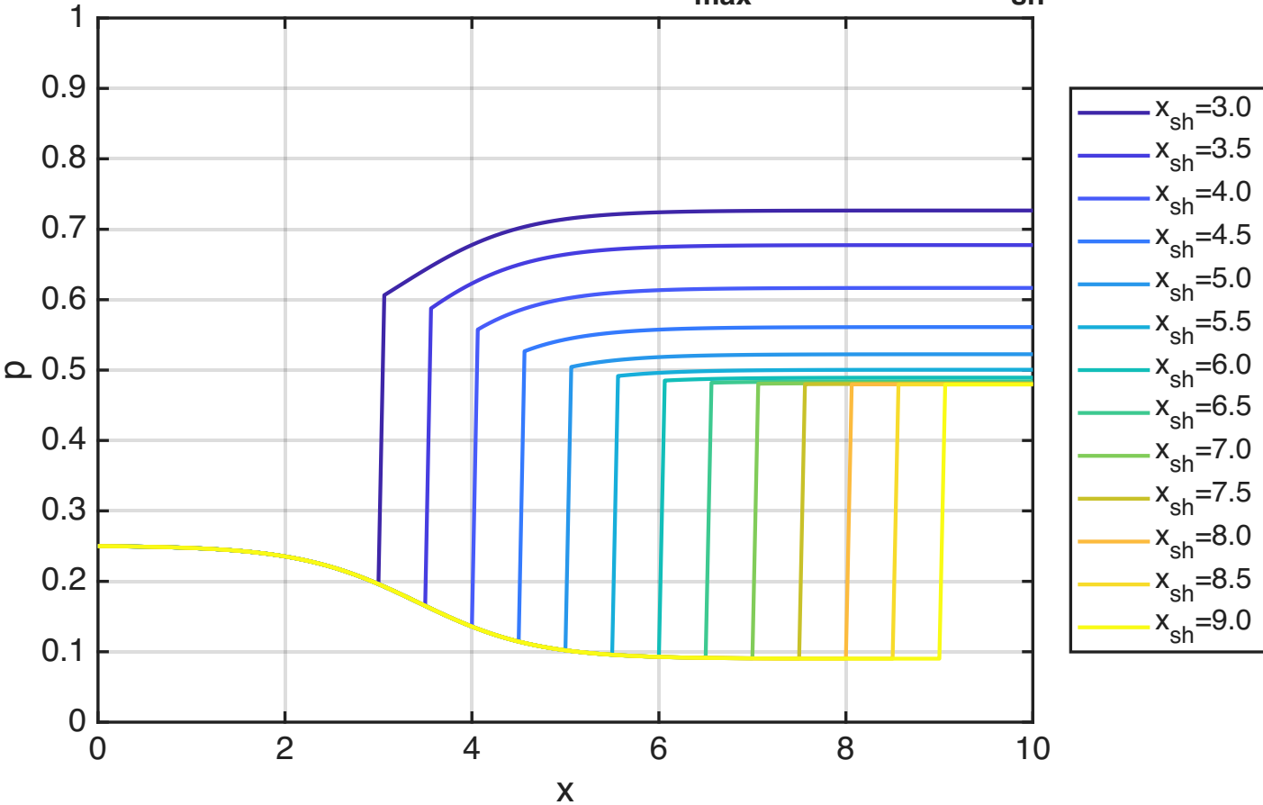
Pressure vs. x (predictor-corrector, j_{\max}=161 , varying x_{\text{sh}} )
