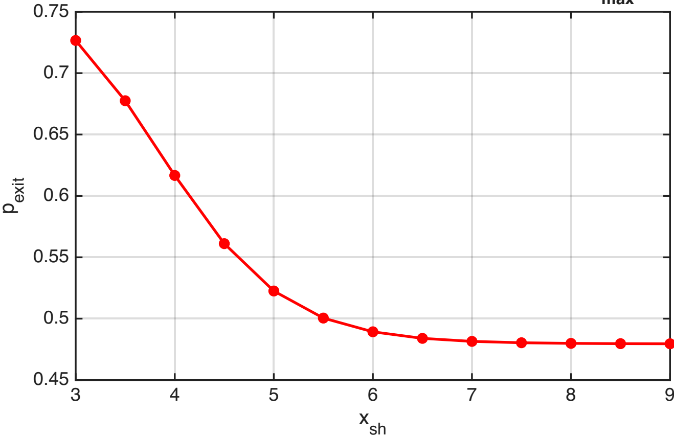
Exit Pressure vs. Shock Location (predictor-corrector, j_{\max}=161 )
