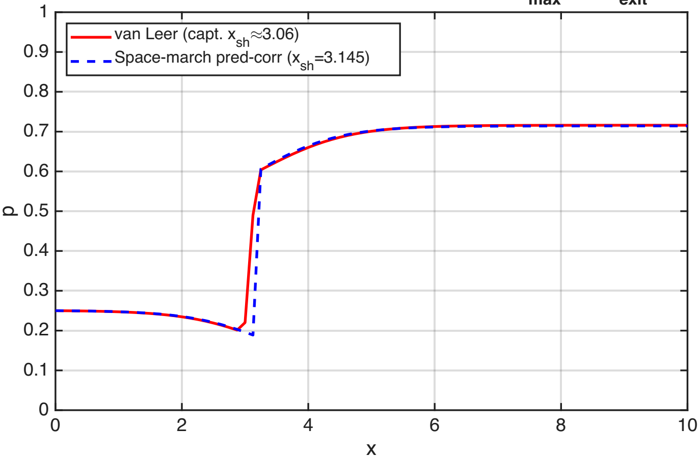
Shock Capturing (van Leer) vs. Space Marching ( j_{\max}=81 , p_{\text{exit}}=1/\gamma )
