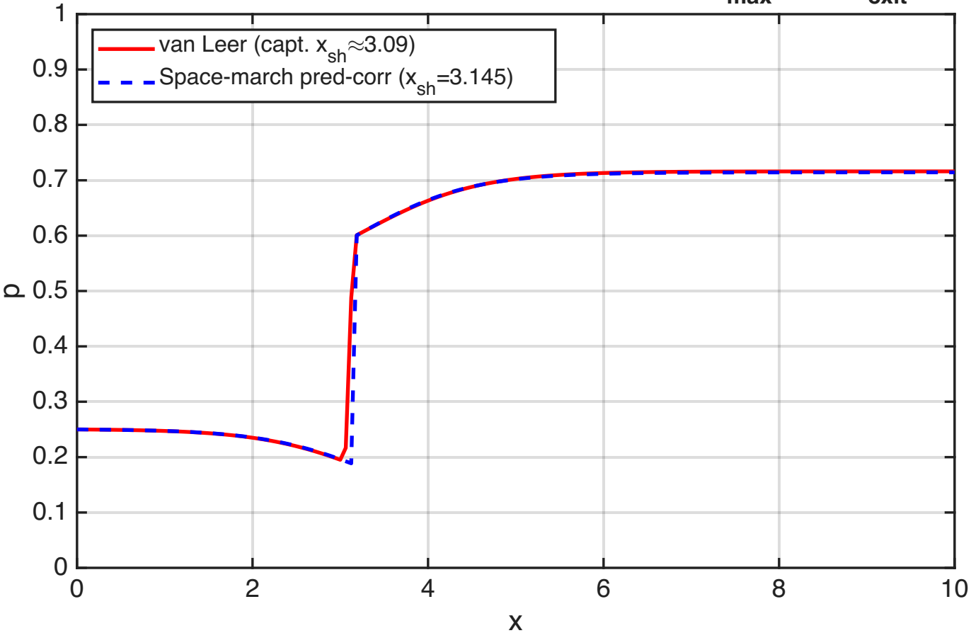
Shock Capturing (van Leer) vs. Space Marching ( j_{\max}=161 , p_{\text{exit}}=1/\gamma )
