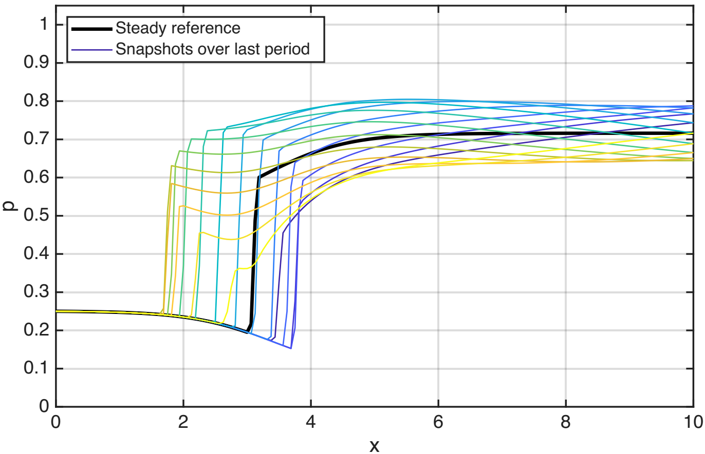
Unsteady pressure envelope (last period): \Delta p_{\text{var}}=0.10 , T=1.00
