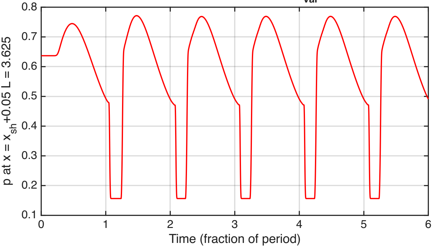
Probe pressure history (6 periods): \Delta p_{\text{var}}=0.10 , T=1.00
