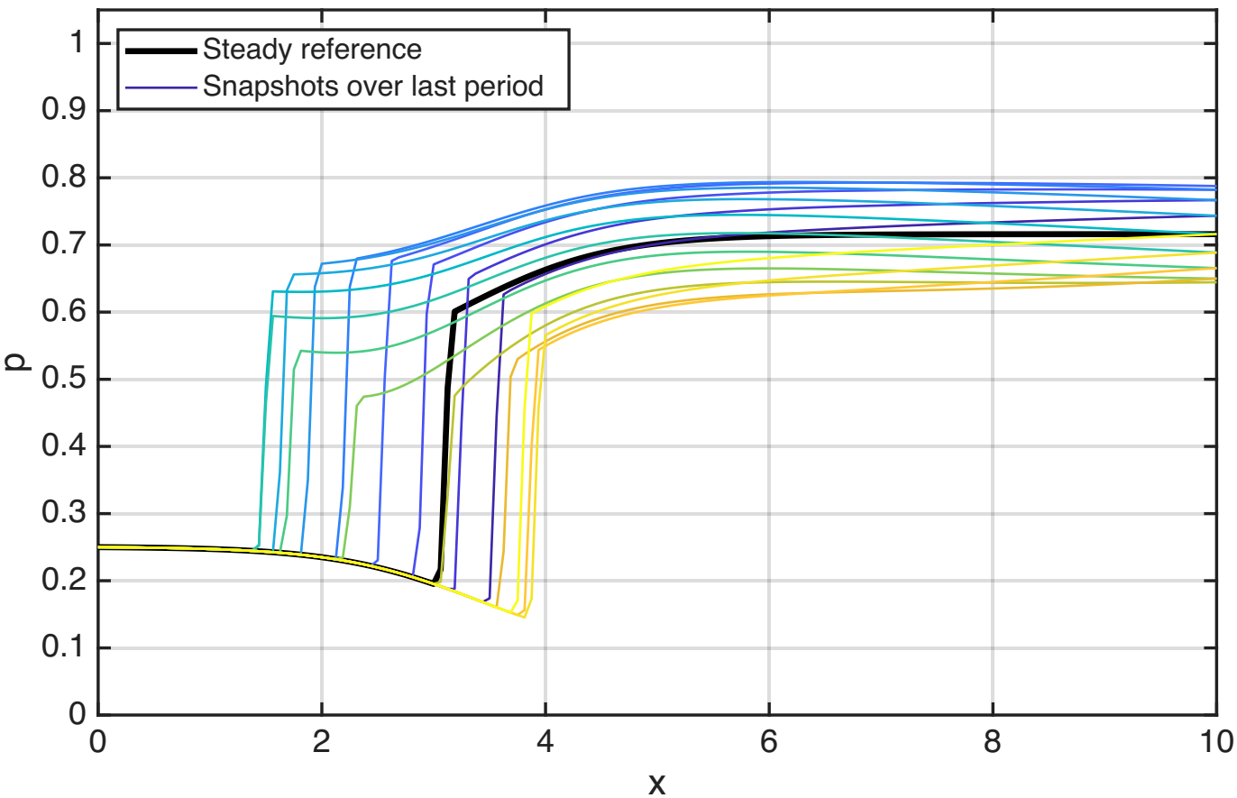
Unsteady pressure envelope (last period): \Delta p_{\text{var}}=0.10 , T=2.00
