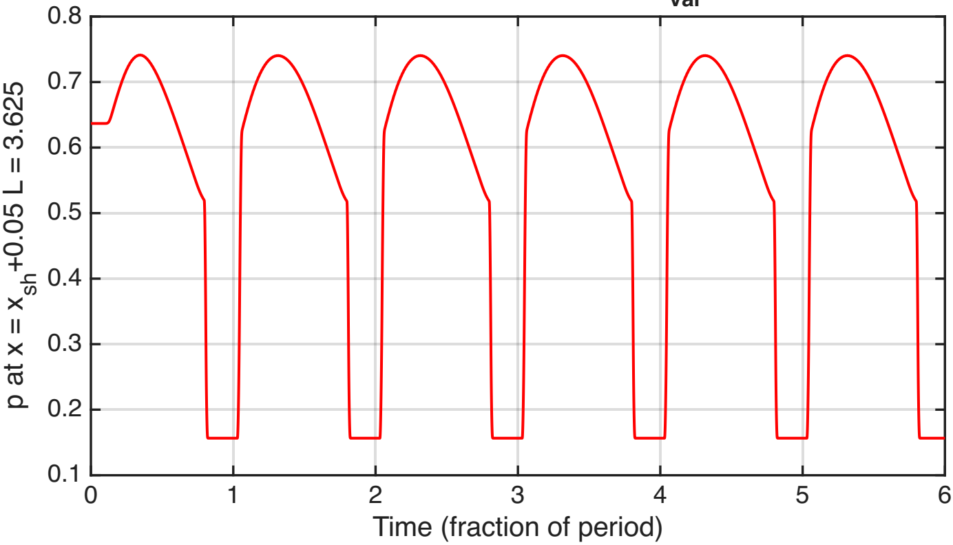
Probe pressure history (6 periods): \Delta p_{\text{var}}=0.10 , T=2.00
