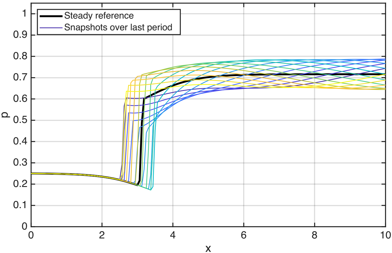
Unsteady pressure envelope (last period): \Delta p_{\text{var}}=0.10 , T=0.50
