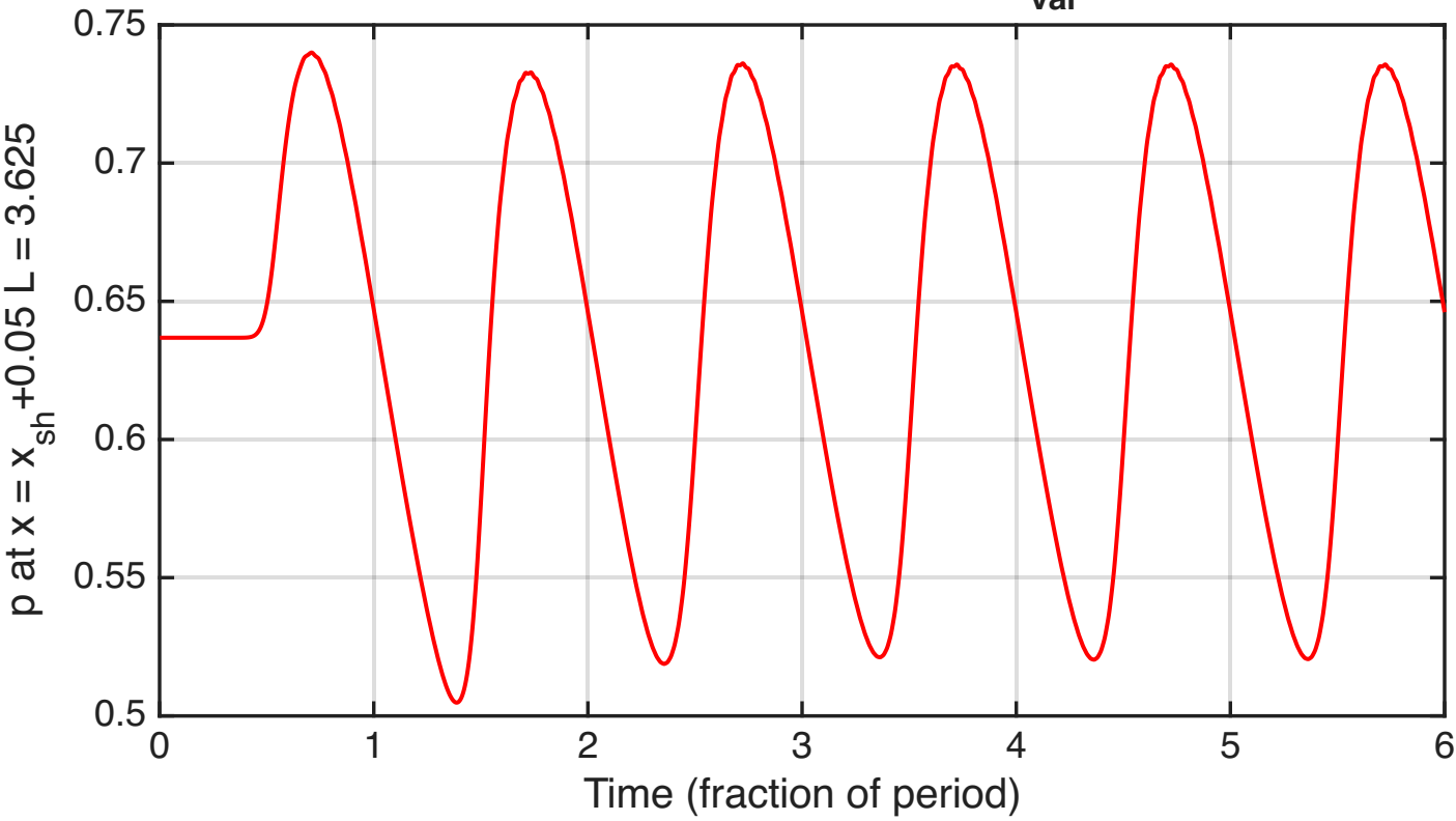
Probe pressure history (6 periods): \Delta p_{\text{var}}=0.10 , T=0.50
