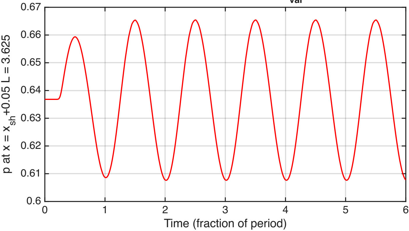
Probe pressure history (6 periods): \Delta p_{\text{var}}=0.02 , T=1.00
